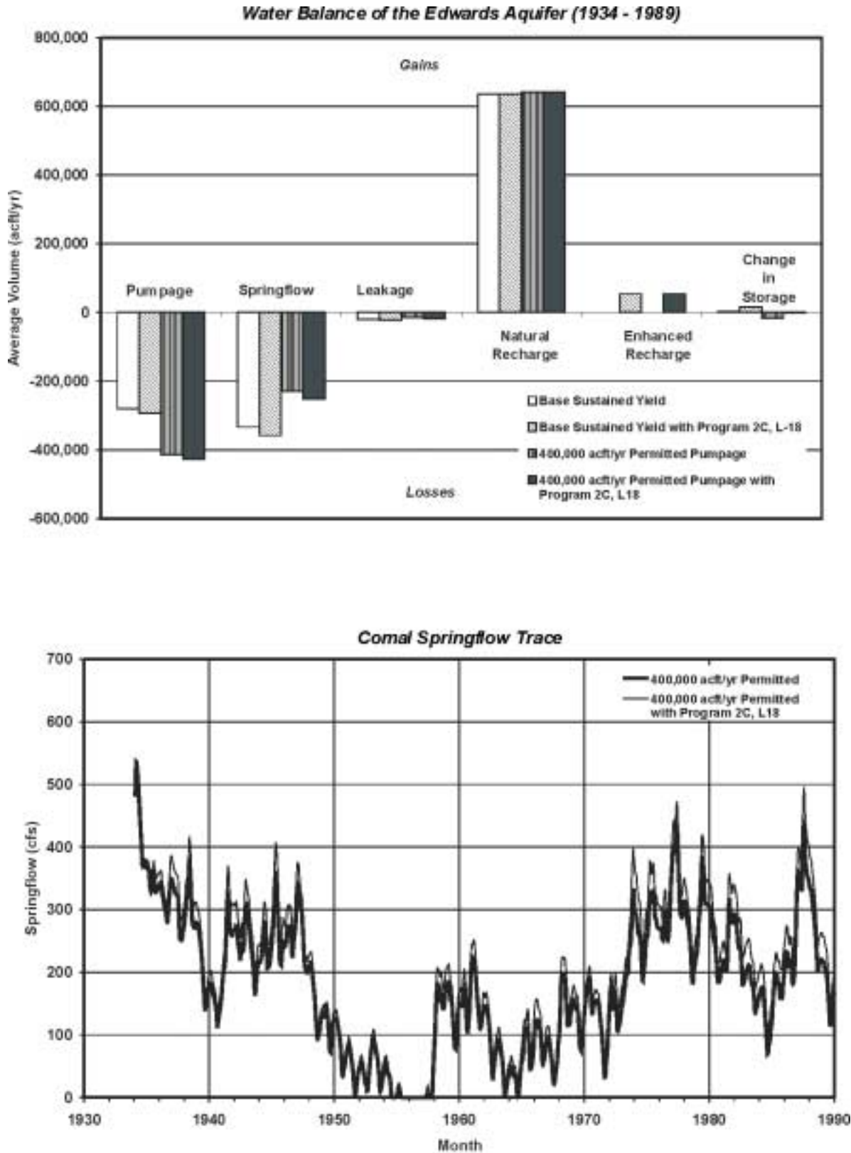
Figure 2.2-5. Enhanced Recharge from Type 2 Recharge Projects — Program 2C
