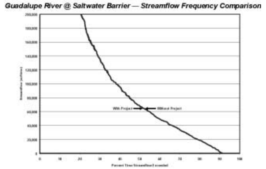
Figure 2.3-5. Medina Lake System Recharge Enhancement Streamflow Comparisons
