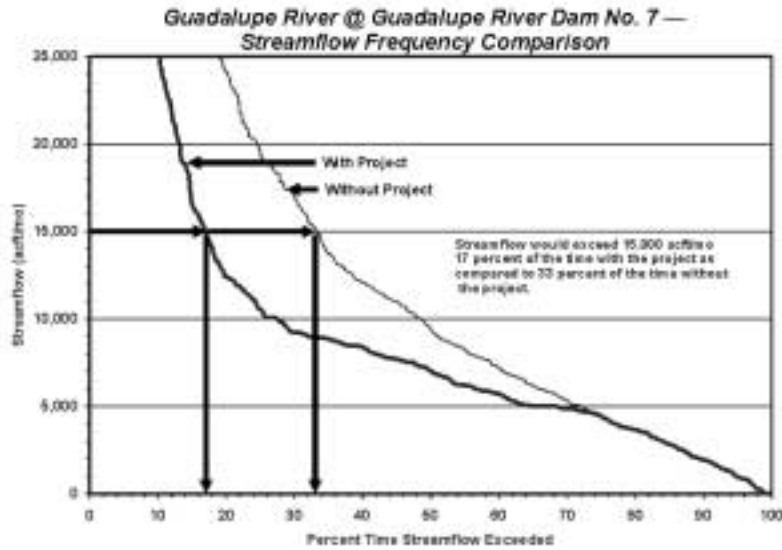
Figure 5.6-3. Guadalupe River Dam No. 7 Streamflow Comparisons
