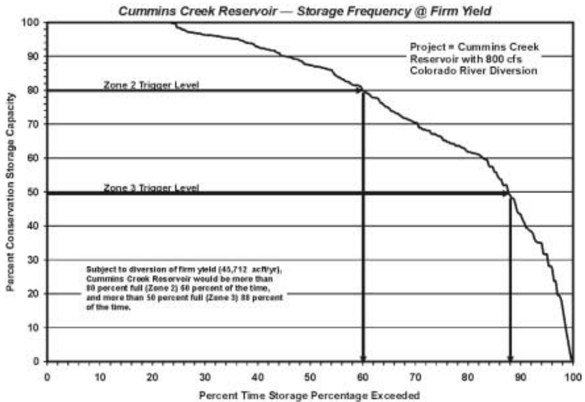
Figure 5.15-5. Cummins Creek Reservoir (Alternative B) Storage Considerations
