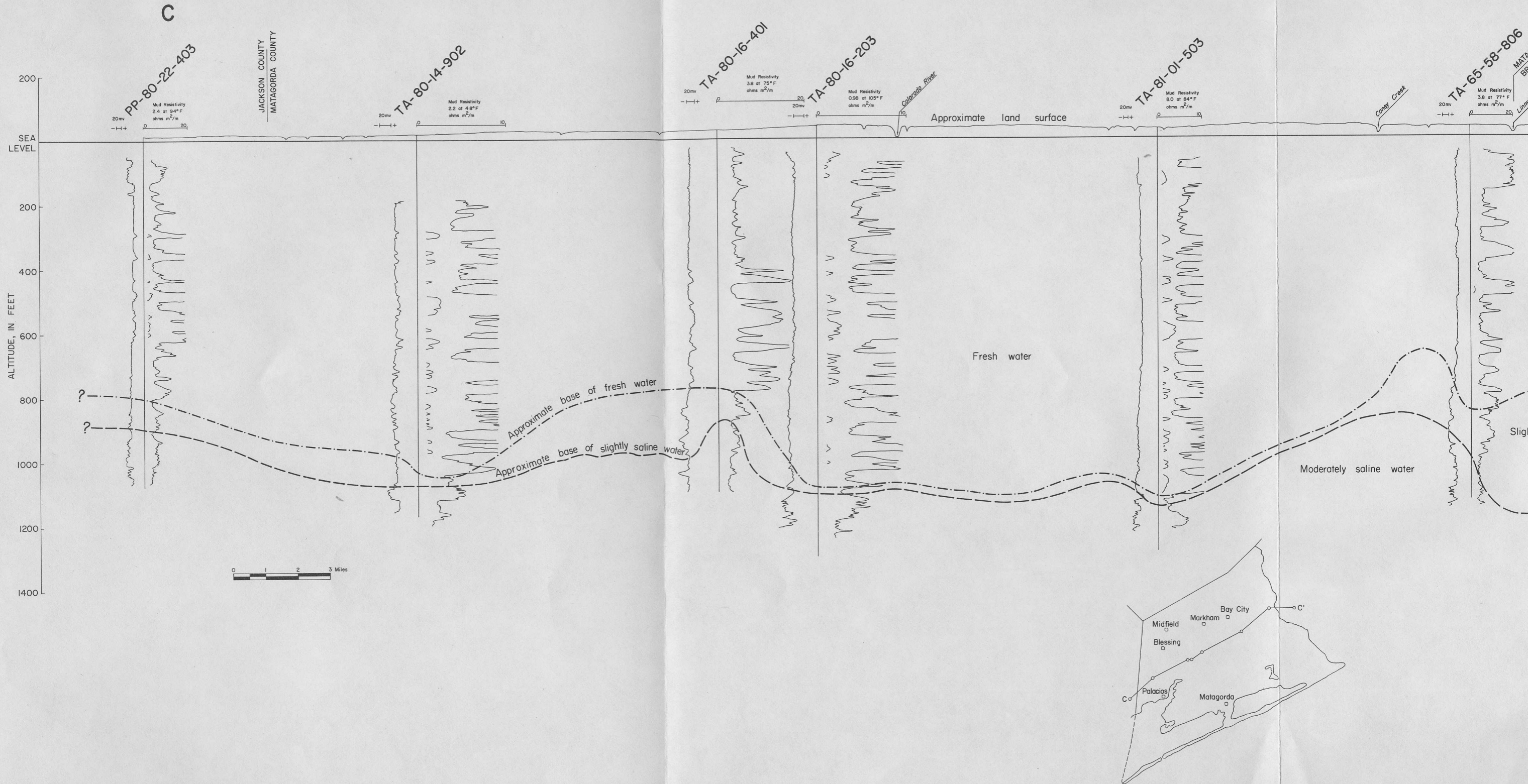
Figure 35 Section C-C' Showing Approximate Bases of Fresh Water and Slightly Saline Water
