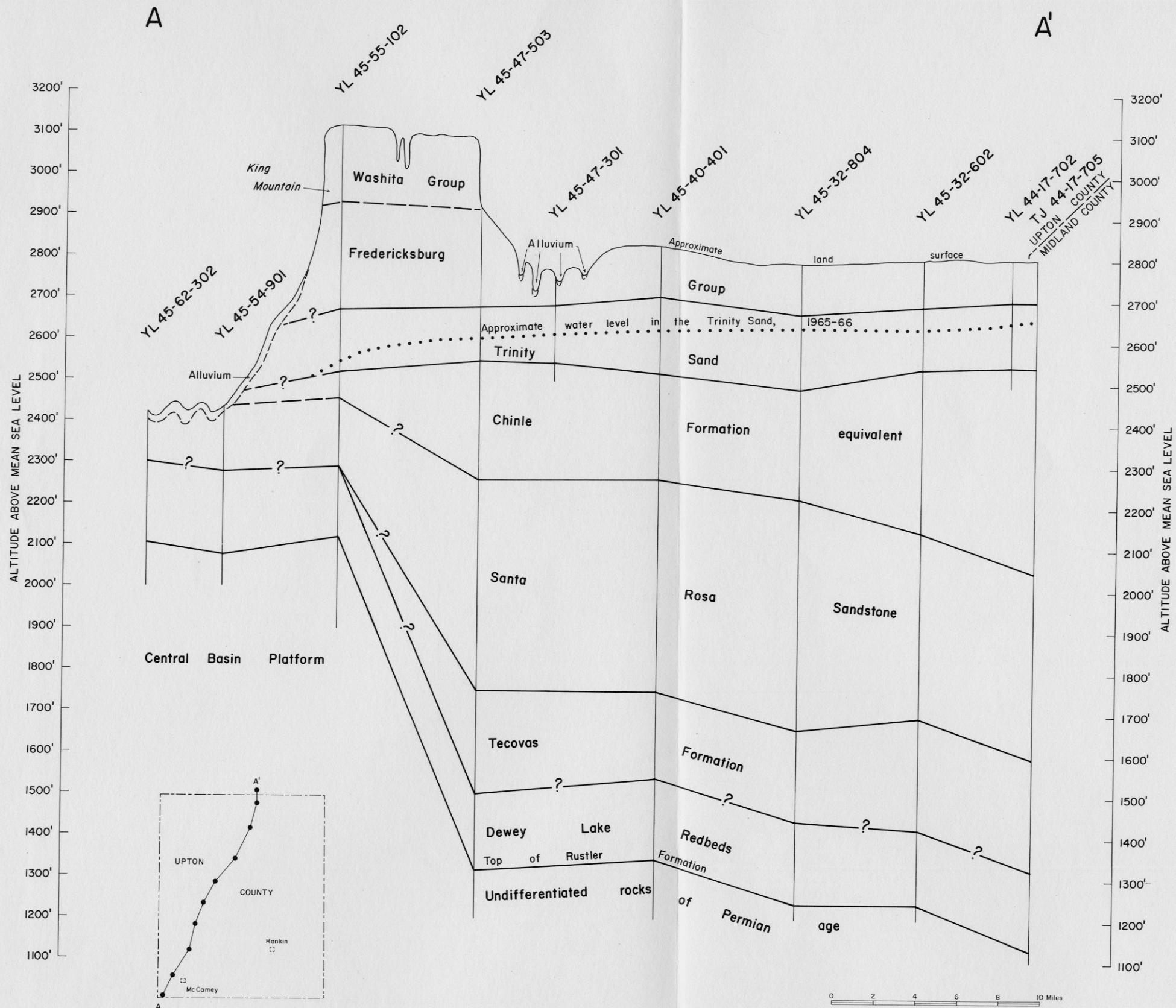
Figure 20 Generalized Geologic Section Along Line A-A'
