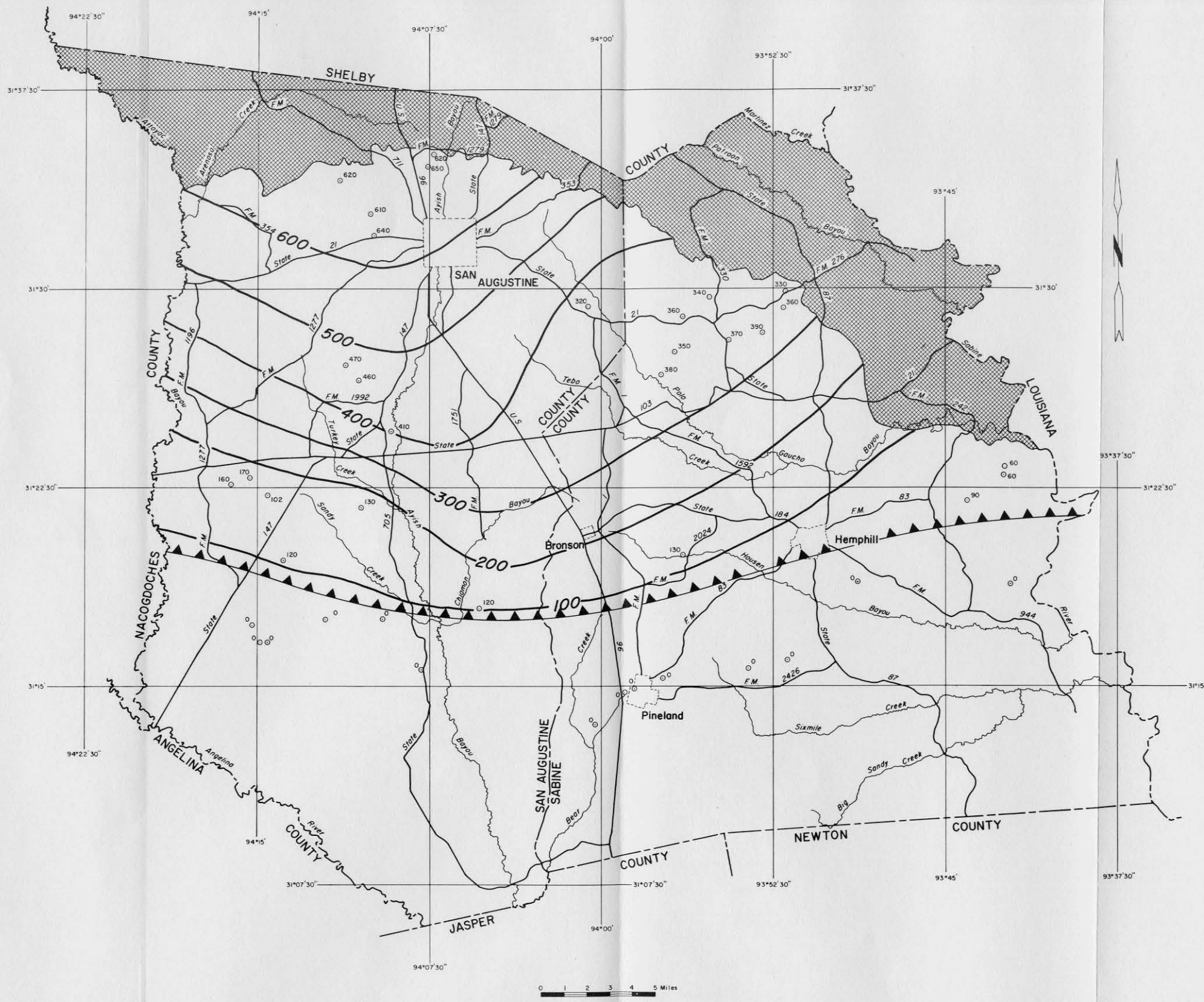
Figure II Approximate Thickness of Sand Containing Fresh to Slightly Saline Water in the Carrizo Sand and Wilcox Group
