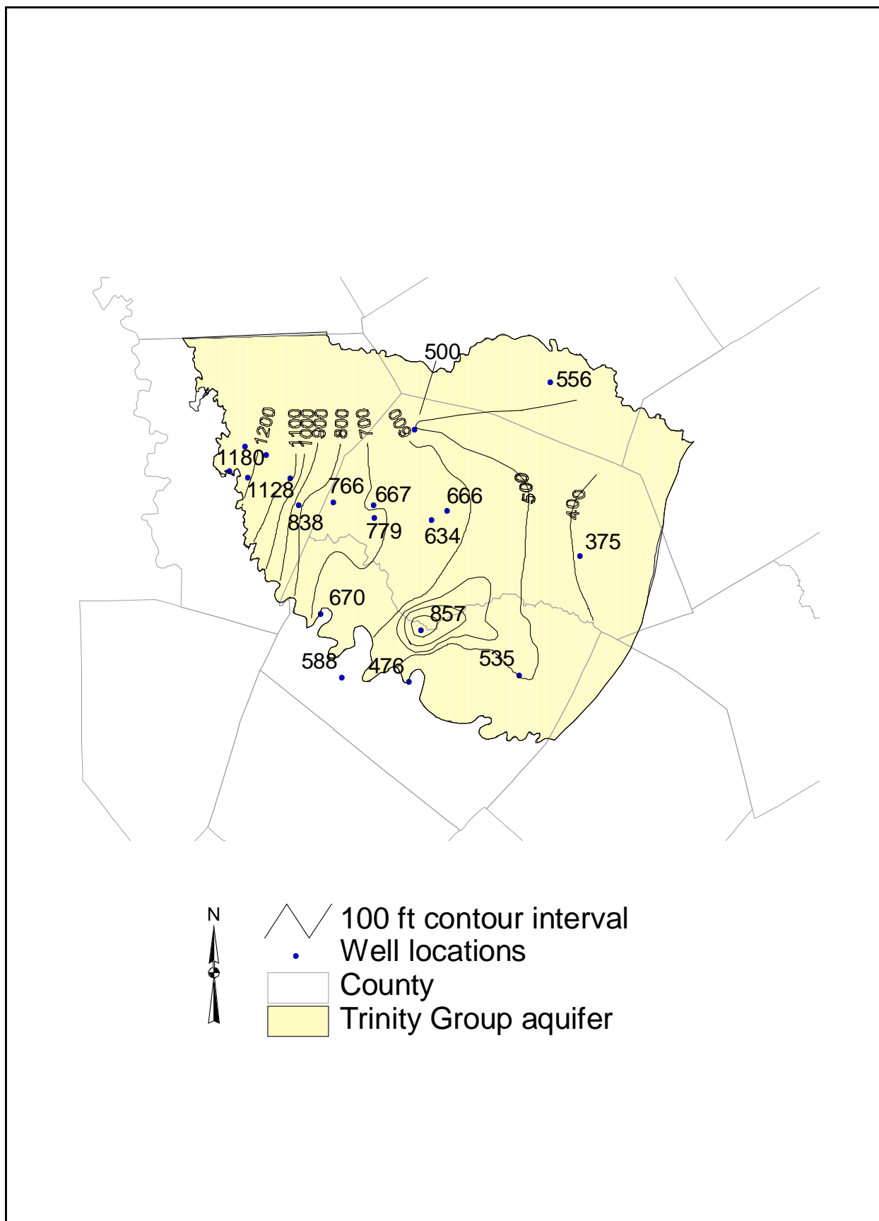
Figure 7. Potentiometric surface map for the Trinity Group aquifer from data collected 1997-1998.
