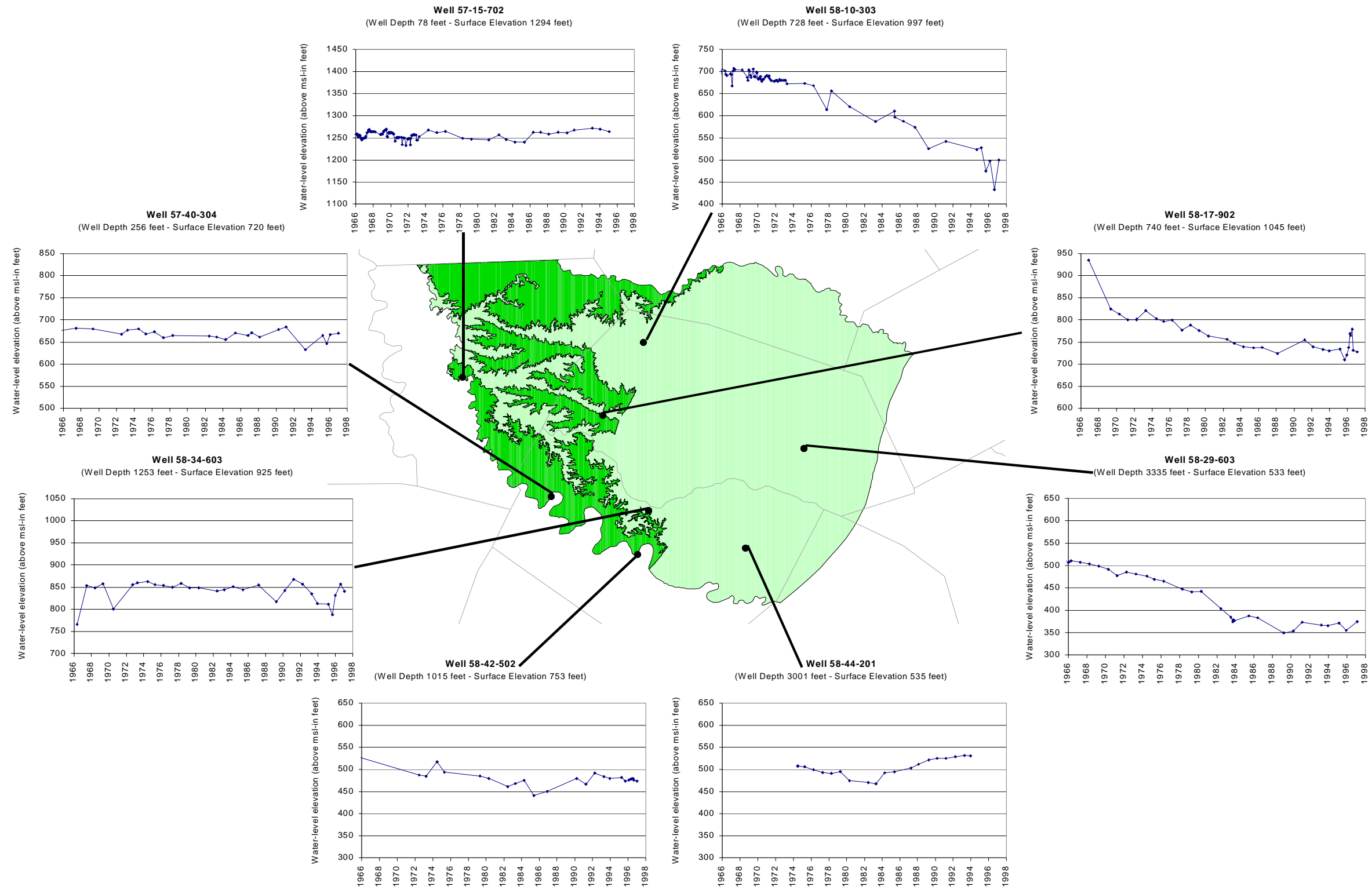
Figure 6. Water-level hydrographs for selected wells completed in the Trinity Group aquifer.
