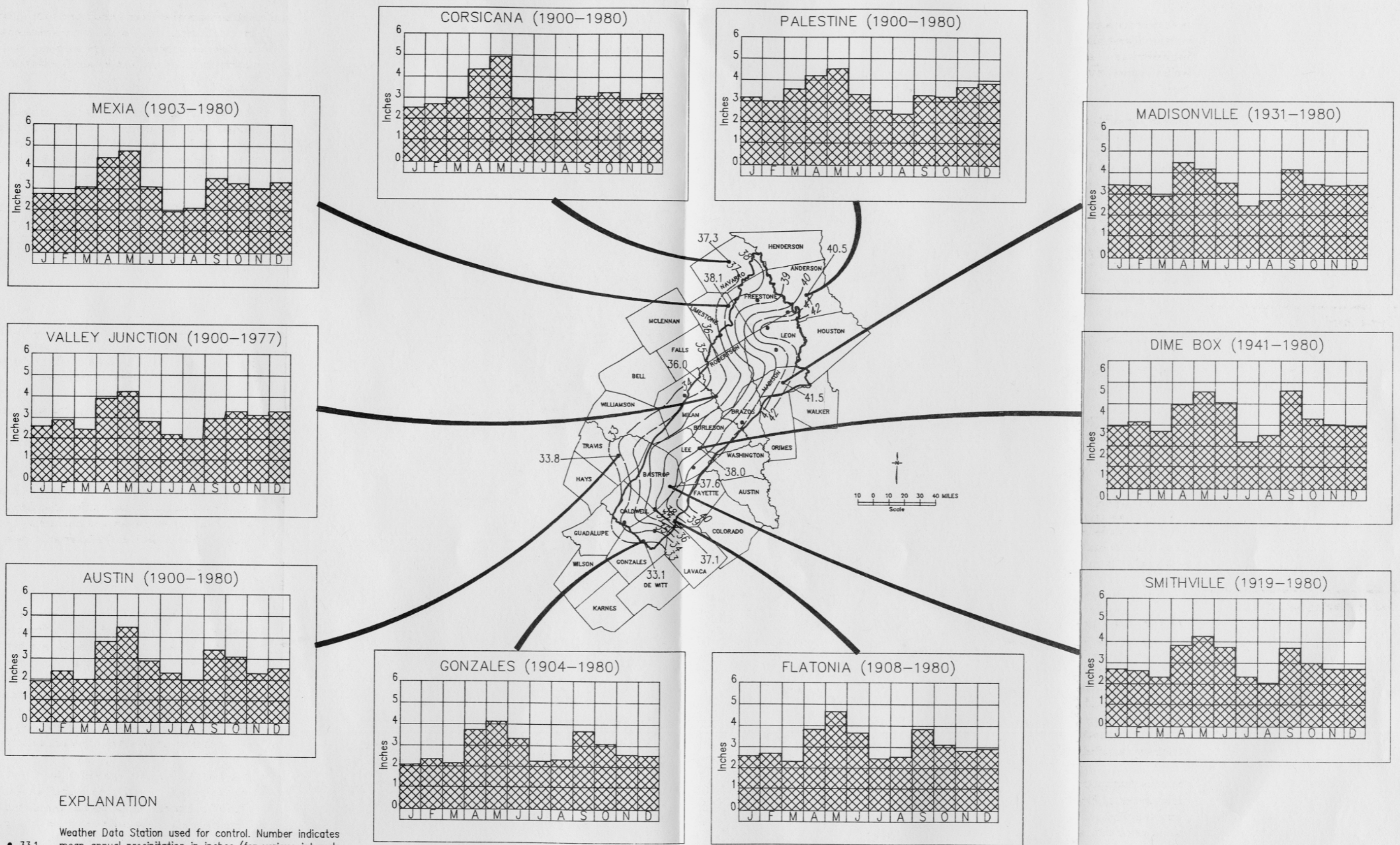
Figure 2 AVERAGE ANNUAL PRECIPITATION, 1900-80, AND AVERAGE MONTHLY PRECIPITATION FOR PERIOD OF RECORD AT SELECTED STATIONS
