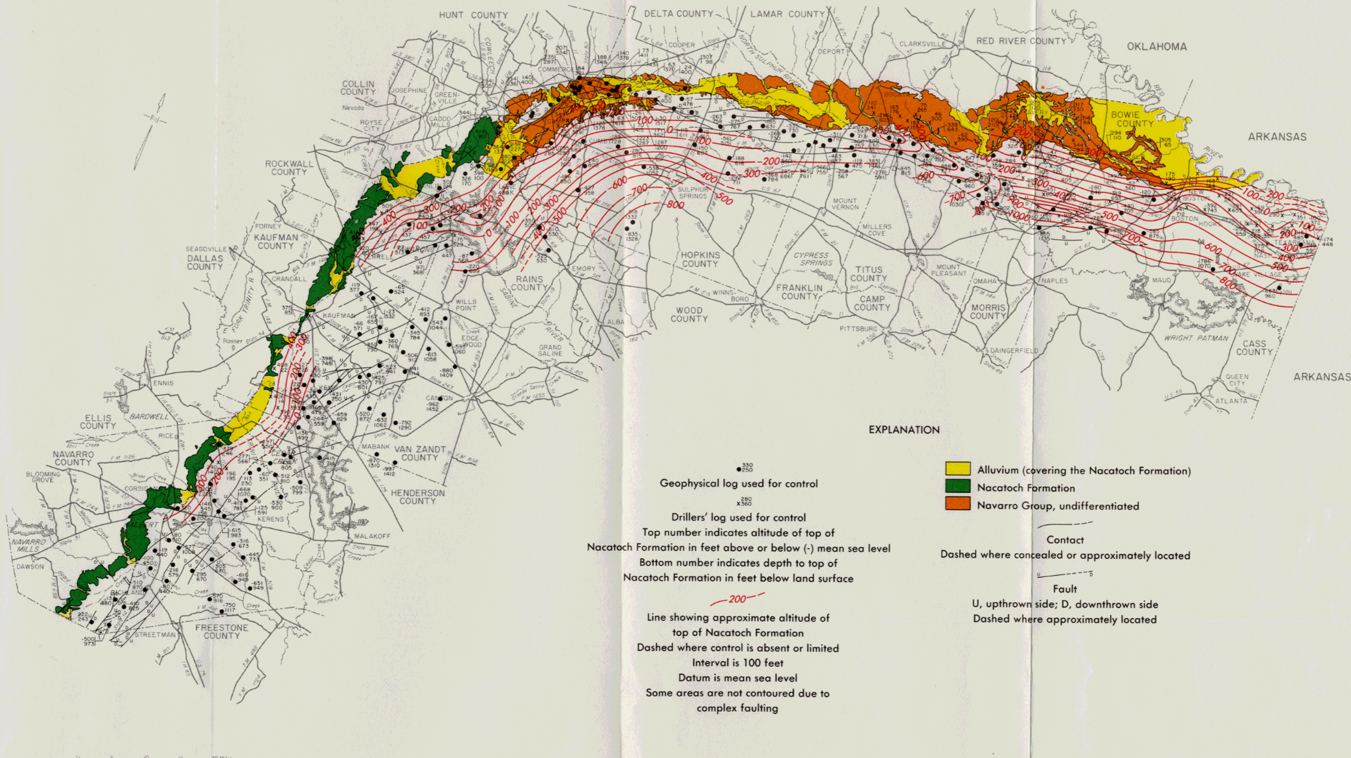
Figure 5 Approximate Altitude of and Depth to the Top of the Nacatoch Formation or Upper Navarro Marl
