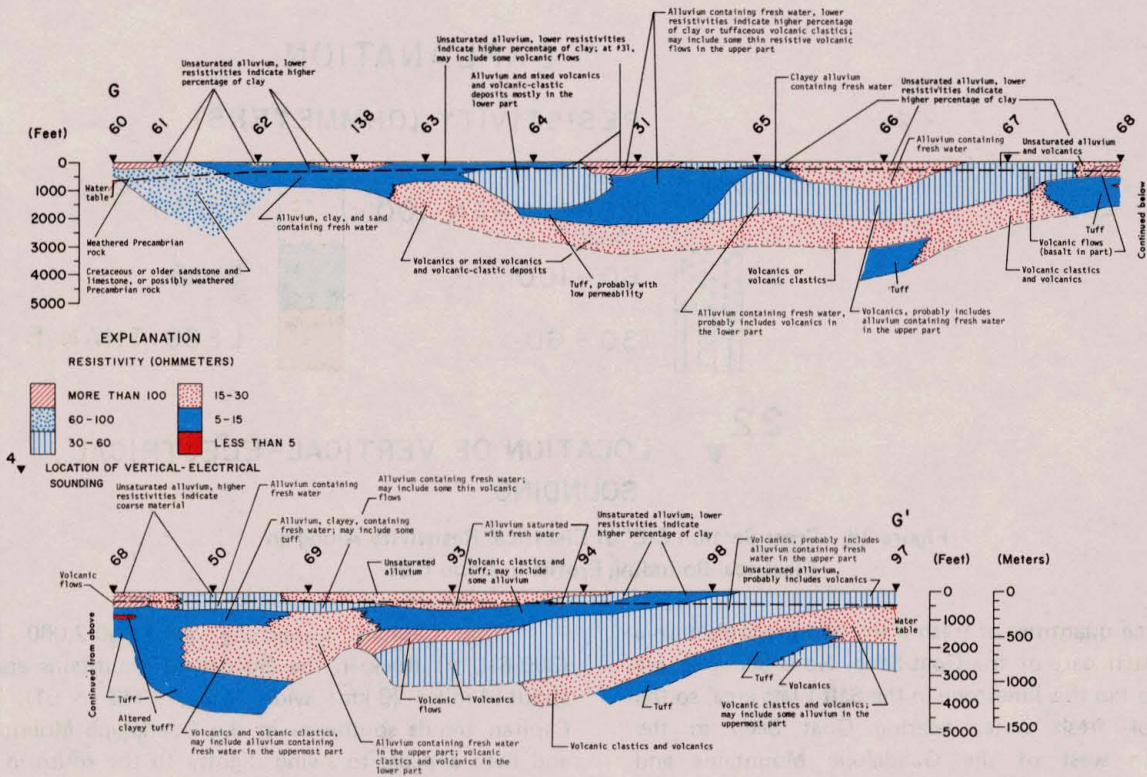
Figure 3f.—Cross Section G-G' of Electrical Resistivity Along an Electrical-Sounding Profile in the Wild Horse, Lobo, and Ryan Flat Areas
