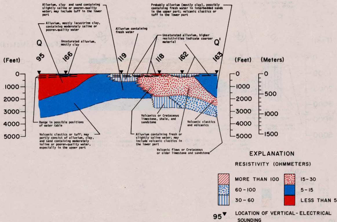
Figure 30.—Cross Section Q-Q' of Electrical Resistivity Along an Electrical-Sounding Profile in the Presidio Bolson
