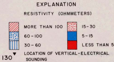
Figure 3j.—Cross Section K-K' of Electrical Resistivity Along an Electrical-Sounding Profile in the Wild Horse Flat Area
