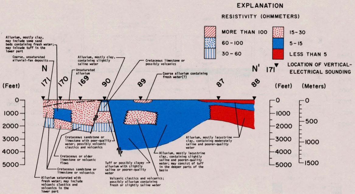
Figure 3l.—Cross Section N-N' of Electrical Resistivity Along an Electrical-Sounding Profile in Red Light Draw
