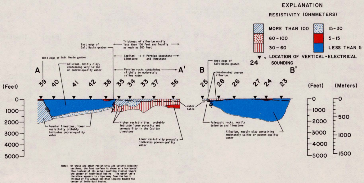
Figure 3a.—Cross Sections A-A' and B-B' of Electrical Resistivity Along Electrical-Sounding Profiles in the Salt Flats Area
