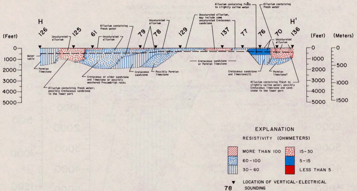
Figure 3g.—Cross Section H-H' of Electrical Resistivity Along an Electrical-Sounding Profile Mostly in the Wild Horse and Michigan Flat Areas
