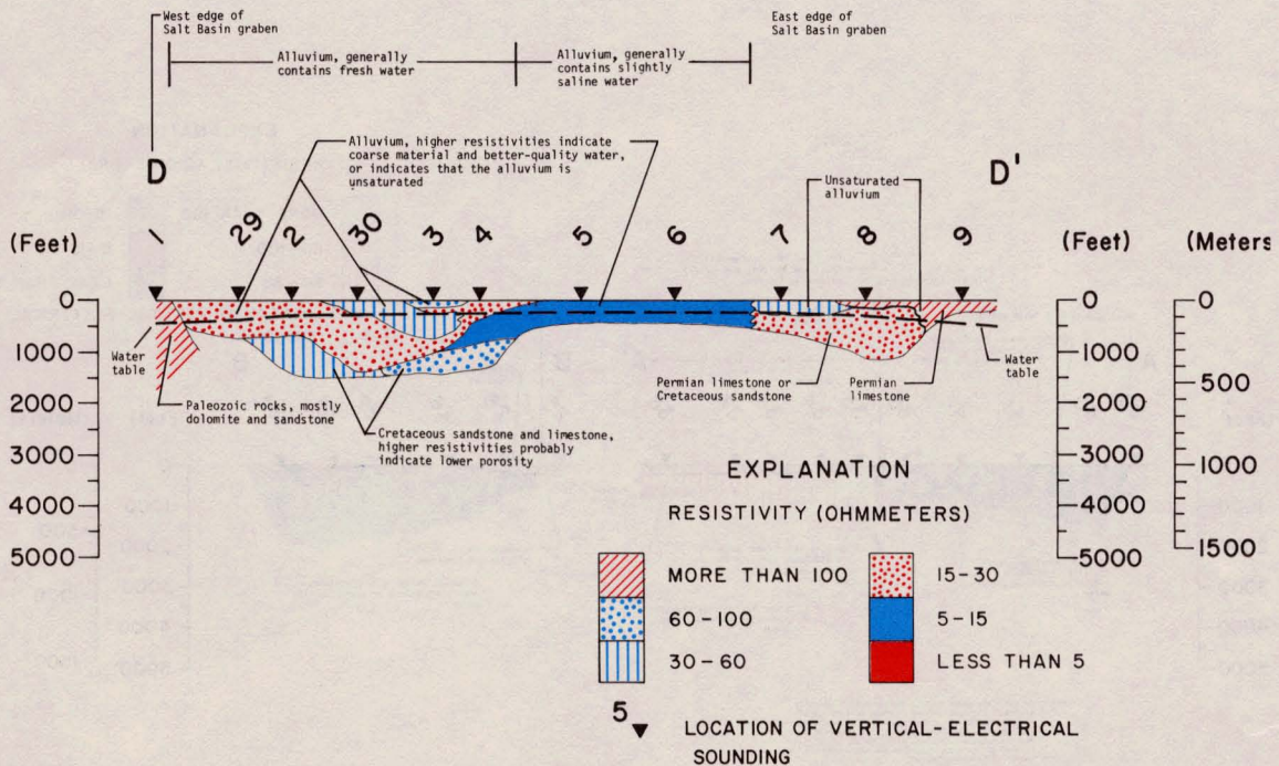
Figure 3c.—Cross Section D-D' of Electrical Resistivity Along an Electrical-Sounding Profile in Wild Horse Flat
