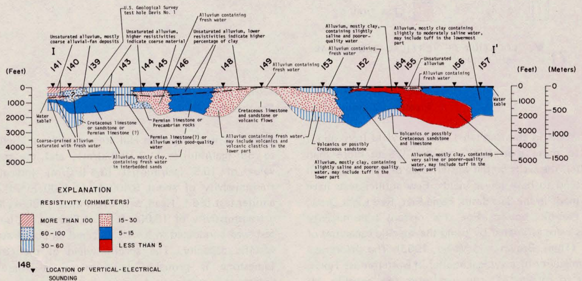
Figure 3h.—Cross Section I-I' of Electrical Resistivity Along an Electrical-Sounding Profile in the Southeastern Eagle Flat and Green River Valley Areas
