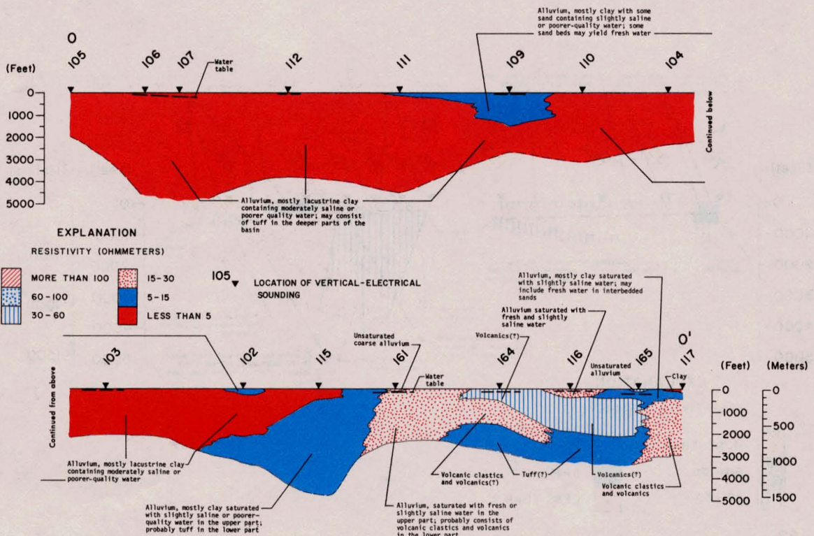
Figure 3m.—Cross Section O-O' of Electrical Resistivity Along an Electrical-Sounding Profile in the Presidio Bolson
