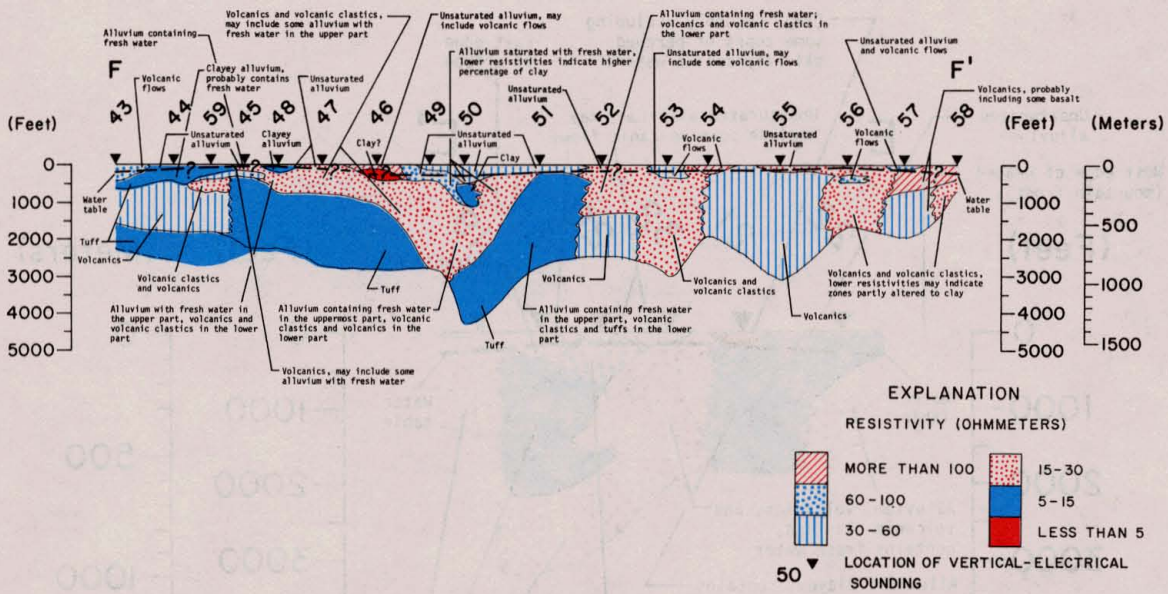
Figure 3e.—Cross Section F-F' of Electrical Resistivity Along an Electrical-Sounding Profile in Ryan Flat
