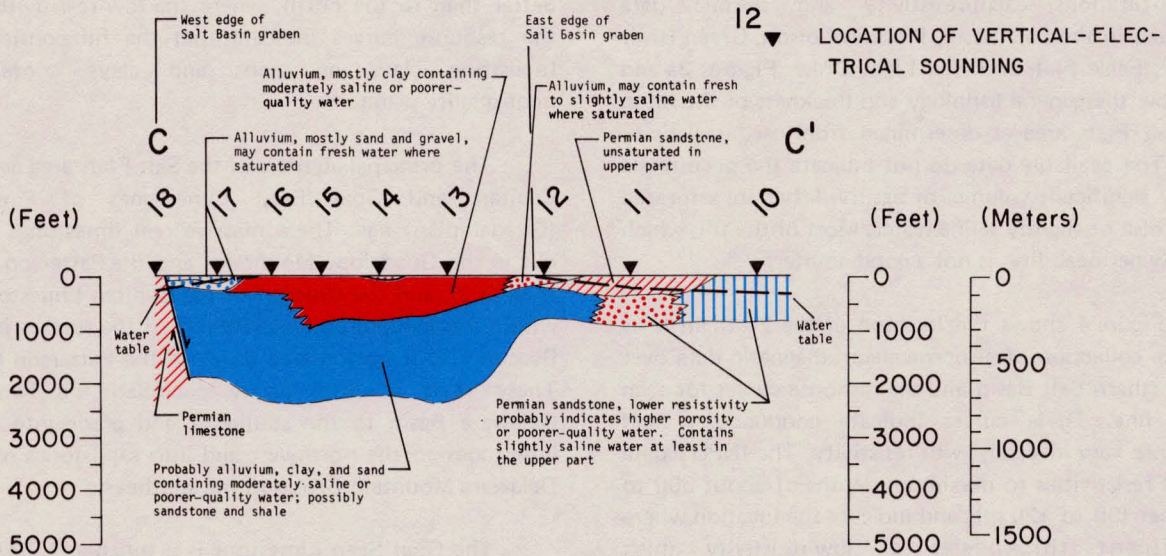
Figure 3b.—Cross Section C-C' of Electrical Resistivity Along an Electrical-Sounding Profile in the Wild Horse and Michigan Flats Area
