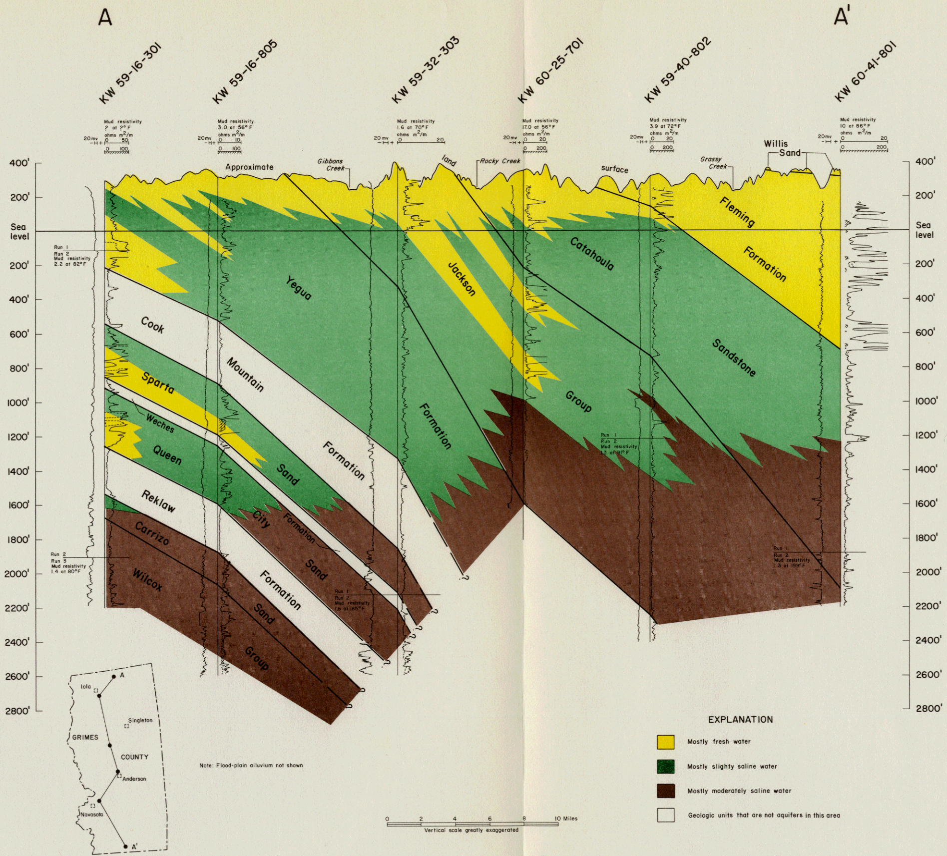
Figure 3 Correlation of Geologic Units and Quality of Water Along Line A-A'
