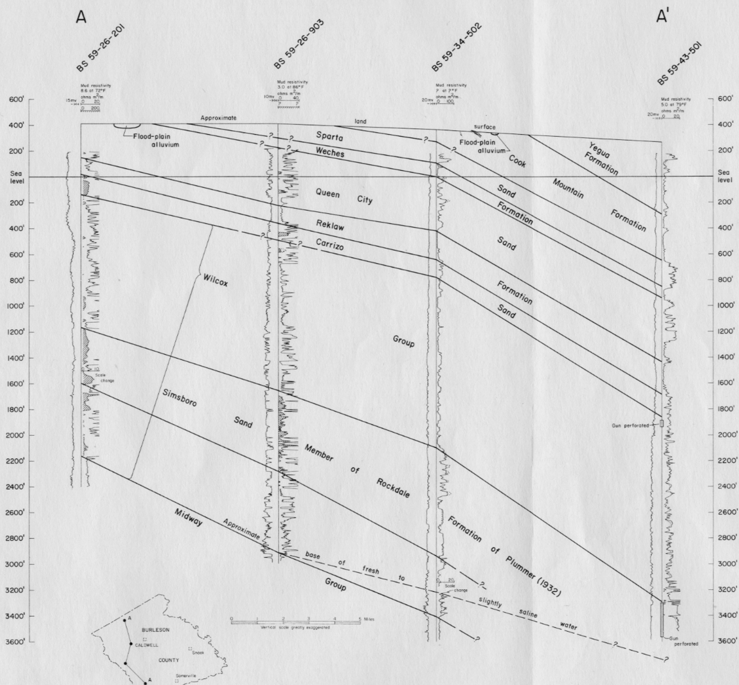
Figure 6 Correlation of Geologic Units Along Line A-A', Burleson County
