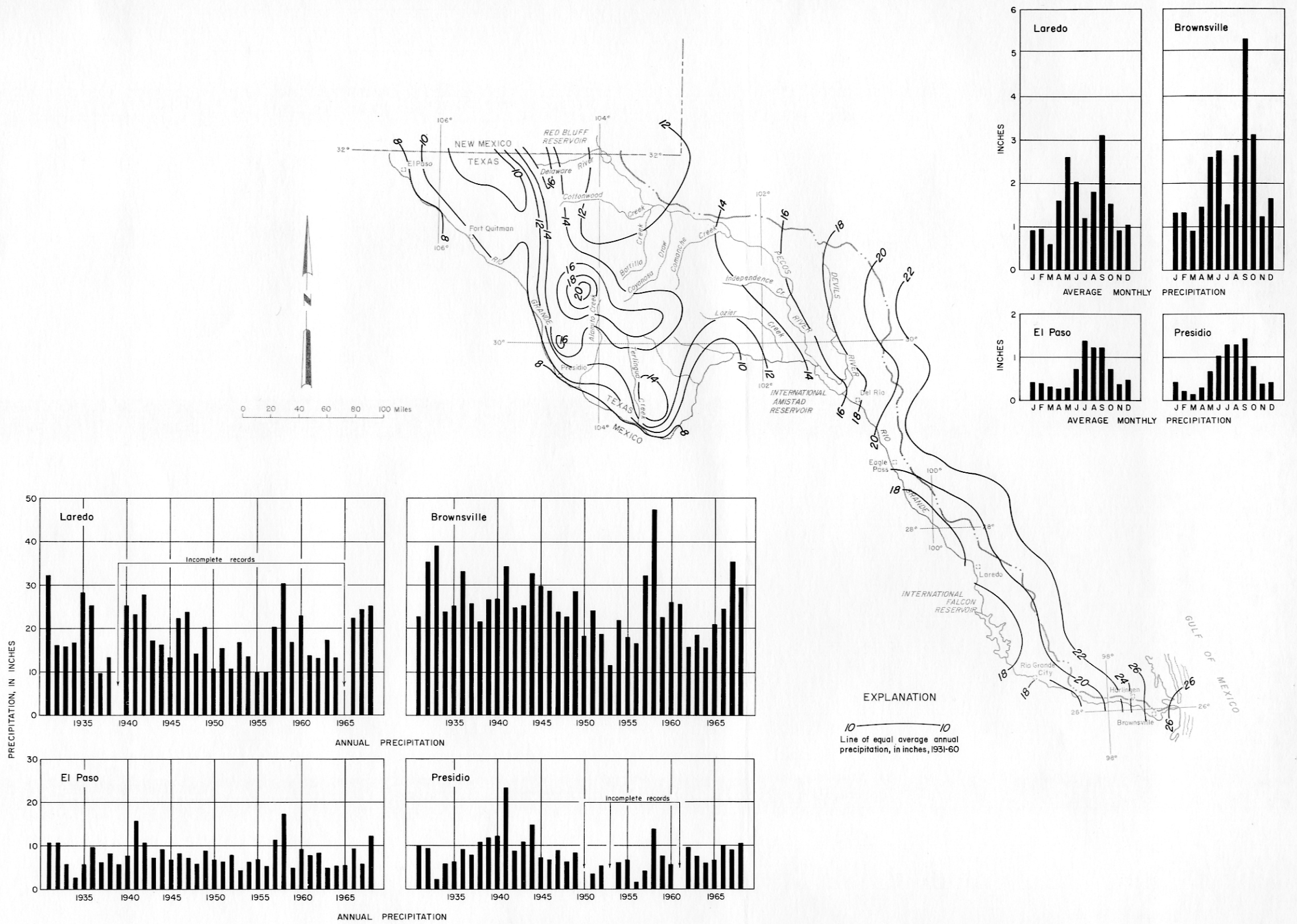
Figure 2 Precipitation in the Texas Part of the Rio Grande Basin
