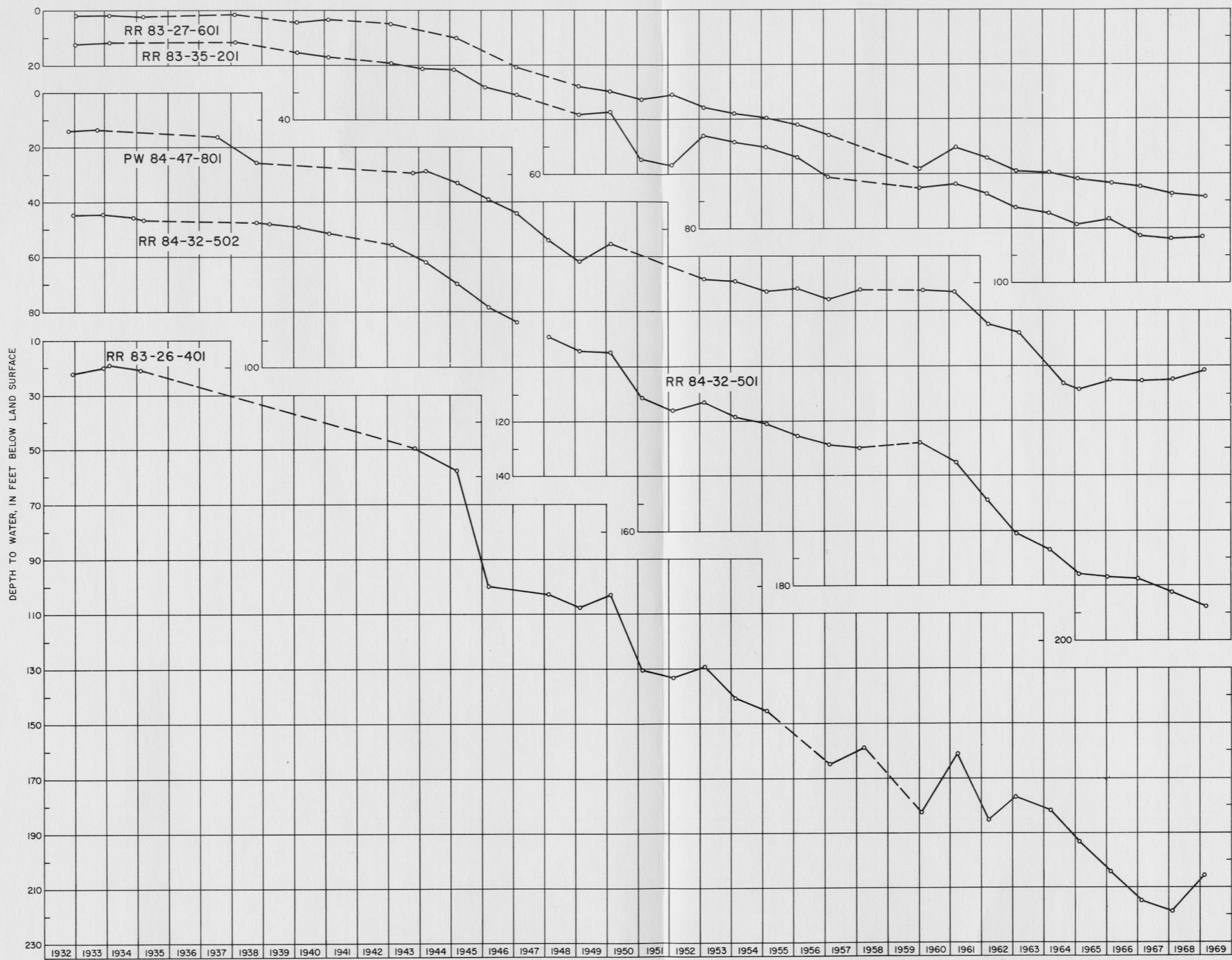
Figure 10 Water Levels in Wells Tapping the Goliad Sand
