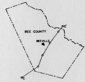
Plate 4 Geologic Section C-C', Live Oak, Bee, and Goliad Counties U.S. Geological Survey in cooperation with the Texas Water Development Board
