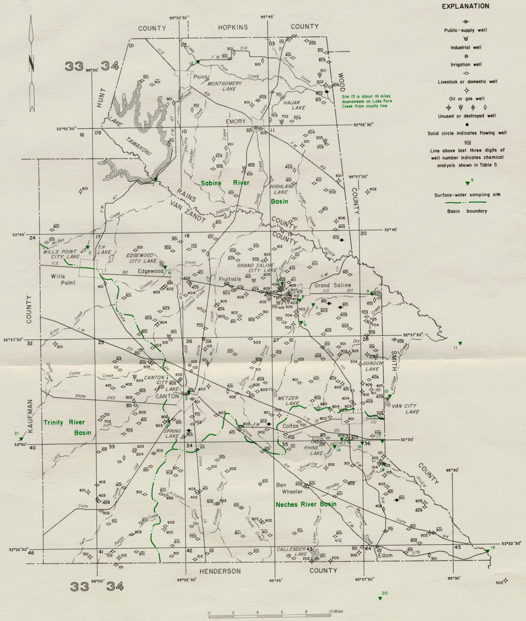
Figure 26 Locations of Wells and Surface-Water Sampling Sites in Rains and Van Zandt Counties and Adjacent Areas
