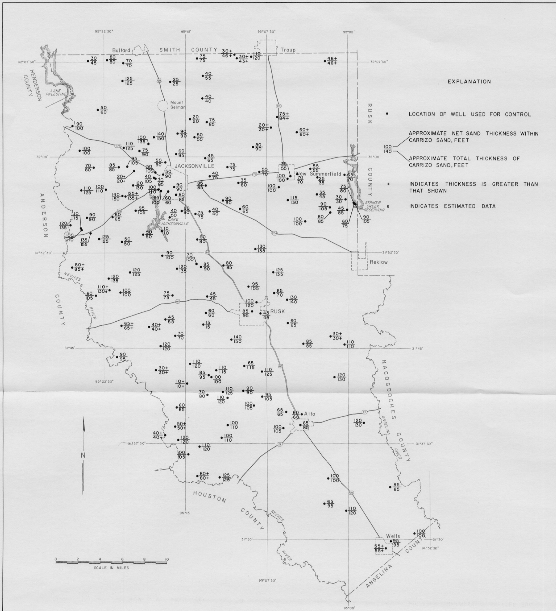
Figure 51 Thickness of Carrizo Sand in Cherokee County
