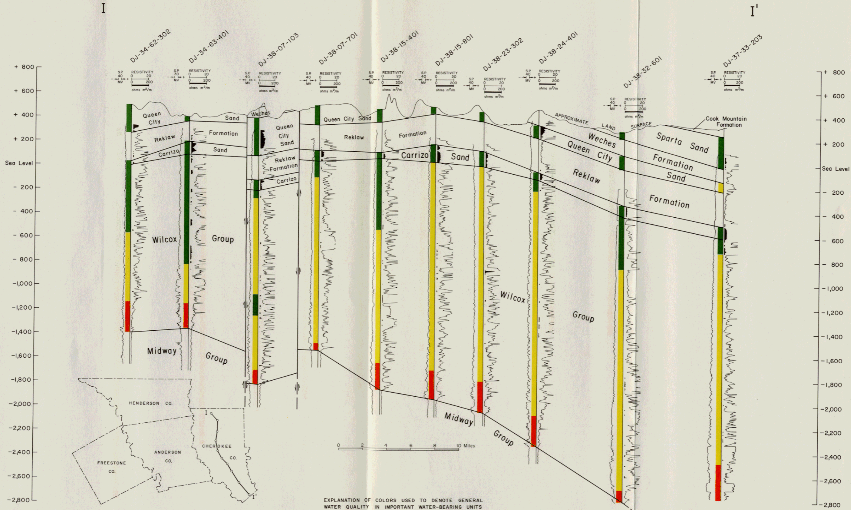
Figure 37 Geologic Section I-I'
