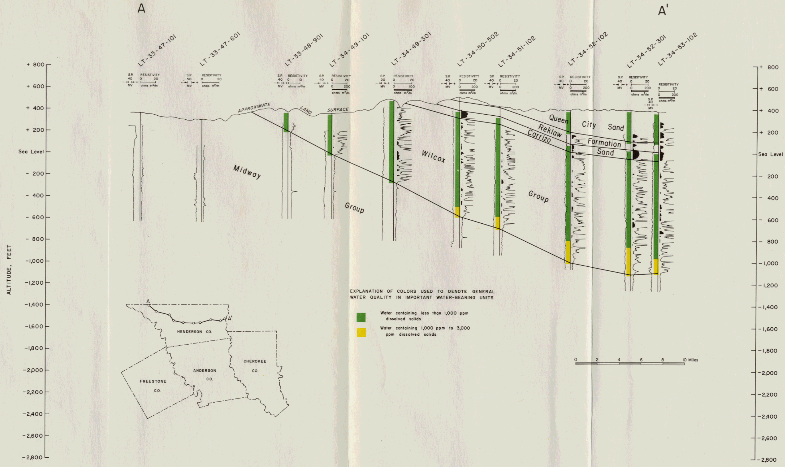
Figure 30 Geologic Section A-A'
