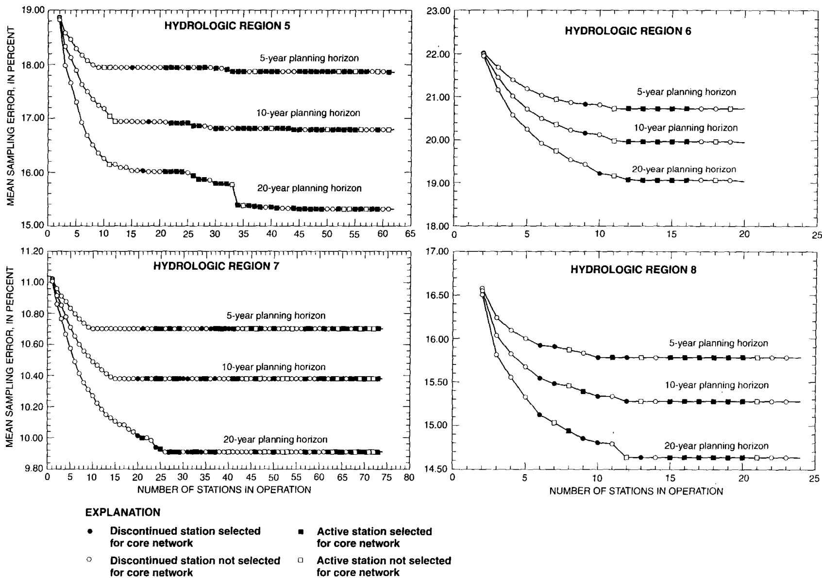
Figure 8. Relation between mean sampling error, number of streamflow-gaging stations, and planning horizon for 25-year peak streamflow in hydrologic regions 5–8.
