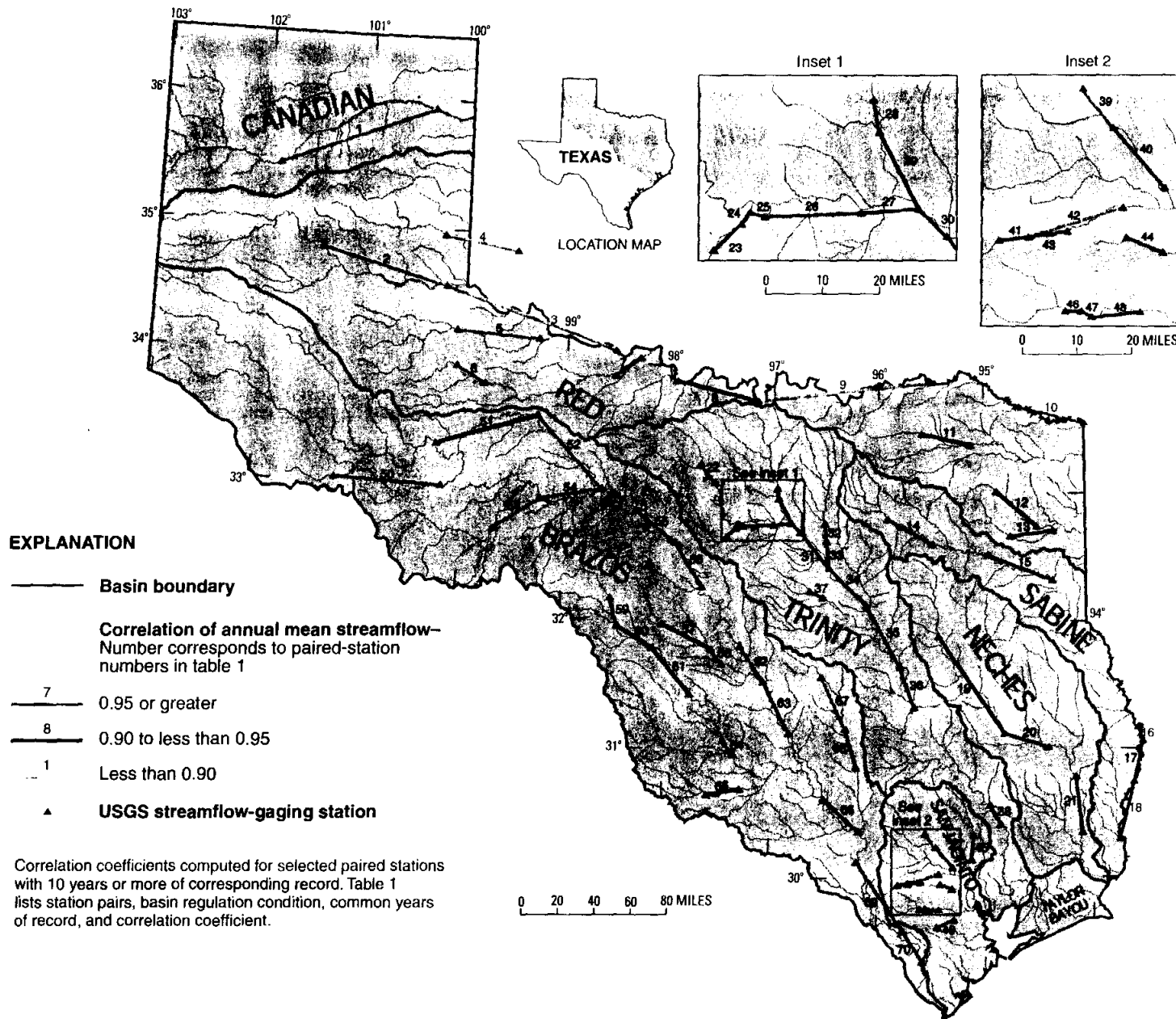
19 Figure 10. Correlation of annual mean streamflow between paired streamflow-gaging stations in north Texas.
