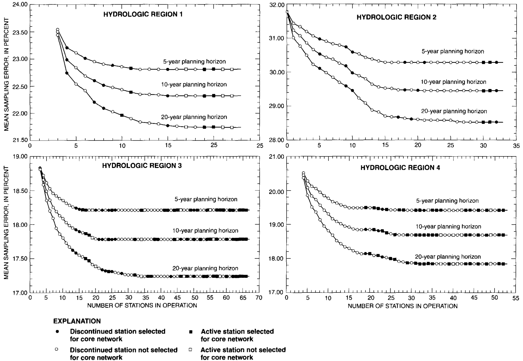
Figure 7. Relation between mean sampling error, number of streamflow-gaging stations, and planning horizon for 25-year peak streamflow in hydrologic regions 1–4.
