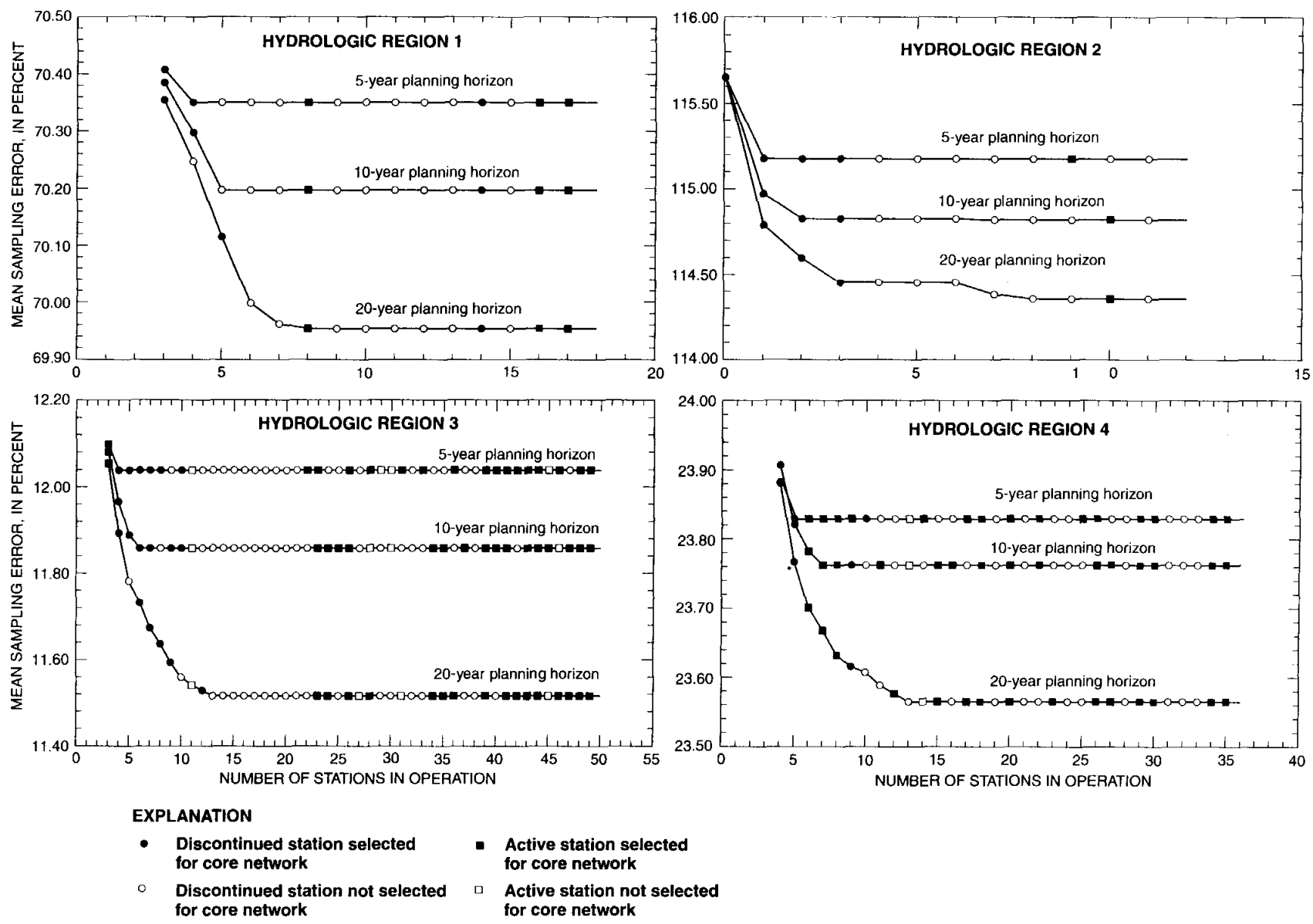
Figure 4. Relation between mean sampling error, number of streamflow-gaging stations, and planning horizon for mean annual streamflow in hydrologic regions 1-4.
