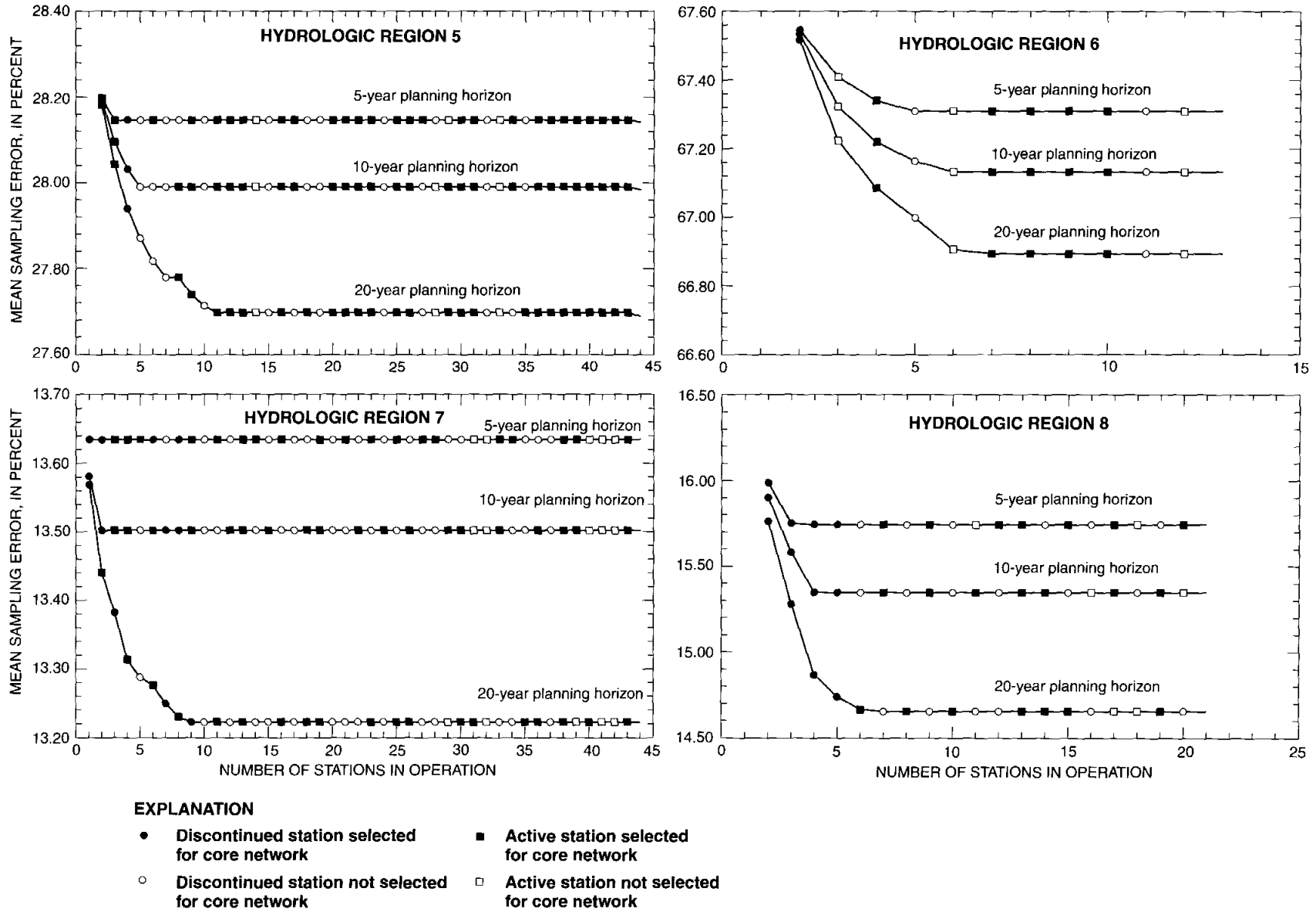
Figure 5. Relation between mean sampling error, number of streamflow-gaging stations, and planning horizon for mean annual streamflow in hydrologic regions 5–8.
