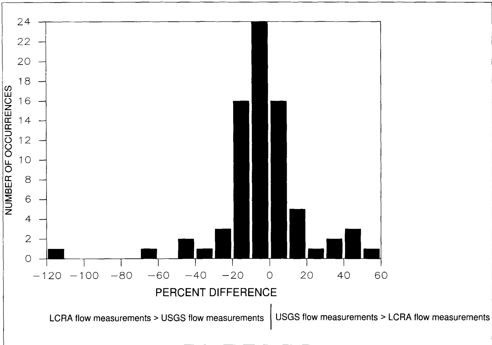
Figure 14. Histogram of percent differences between Lower Colorado River Authority and U.S. Geological Survey flow measurements made more than 1 hour apart, Lakeside district.
