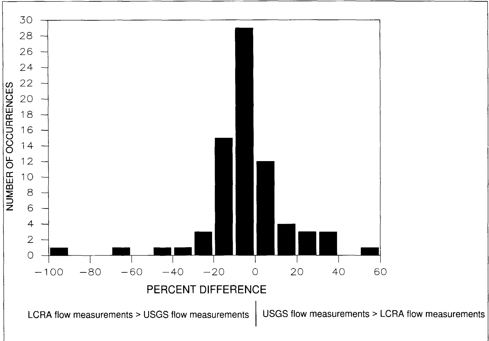
Figure 20. Histogram of percent differences between Lower Colorado River Authority and U.S. Geological Survey flow measurements made more than 1 hour apart, Gulf Coast district.
