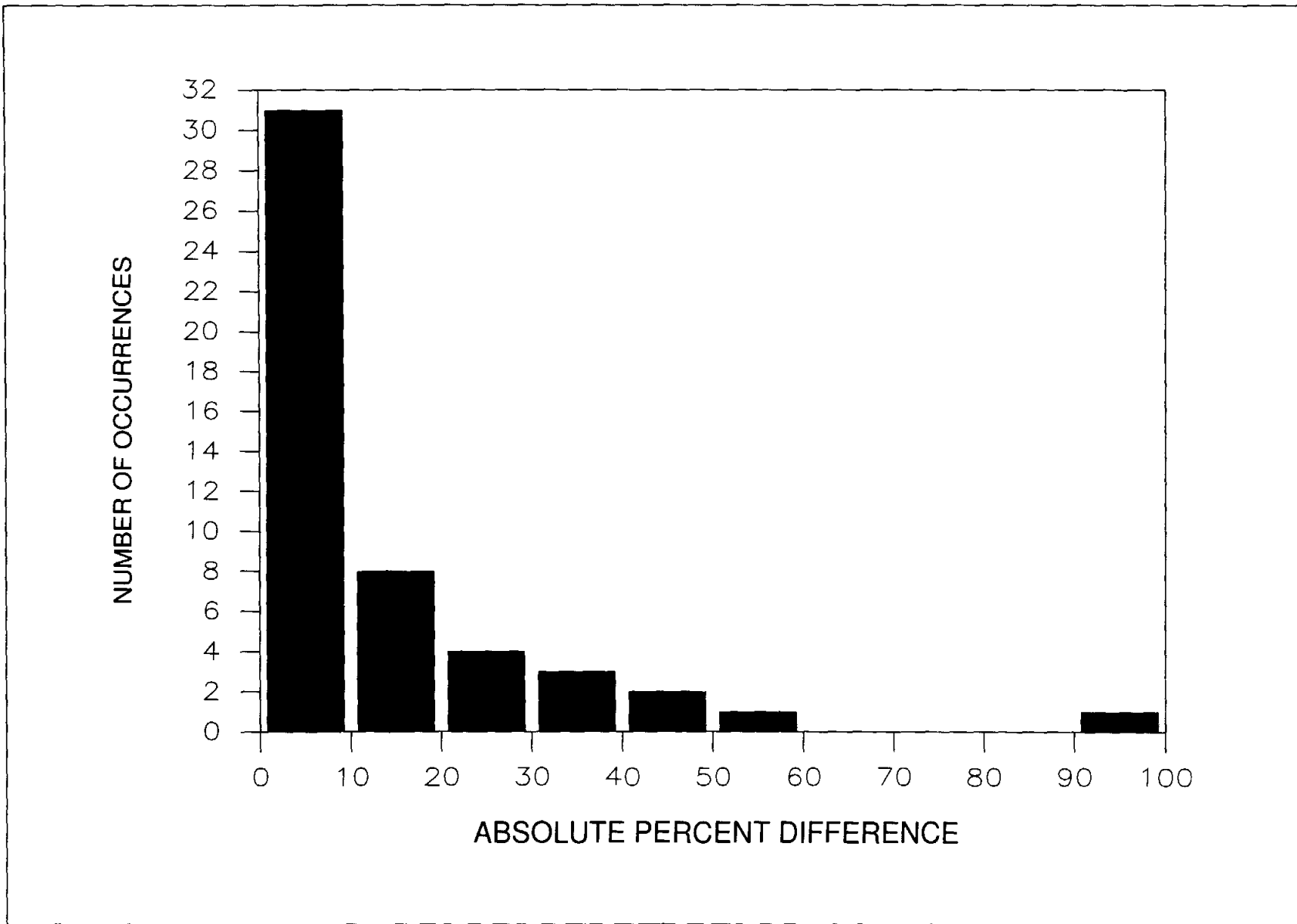
Figure 7. Histogram of absolute percent differences between U.S. Geological Survey-measured morning and afternoon flows, Lakeside district.
