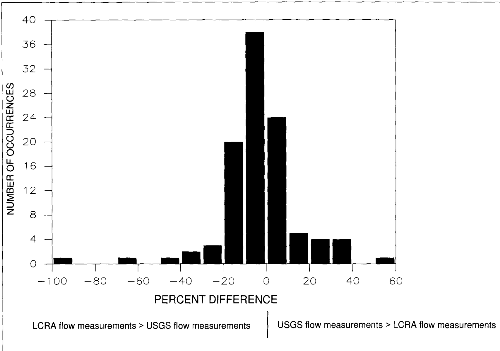
Figure 16. Histogram of percent differences between all Lower Colorado River Authority and U.S. Geological Survey flow measurements, Gulf Coast district.
