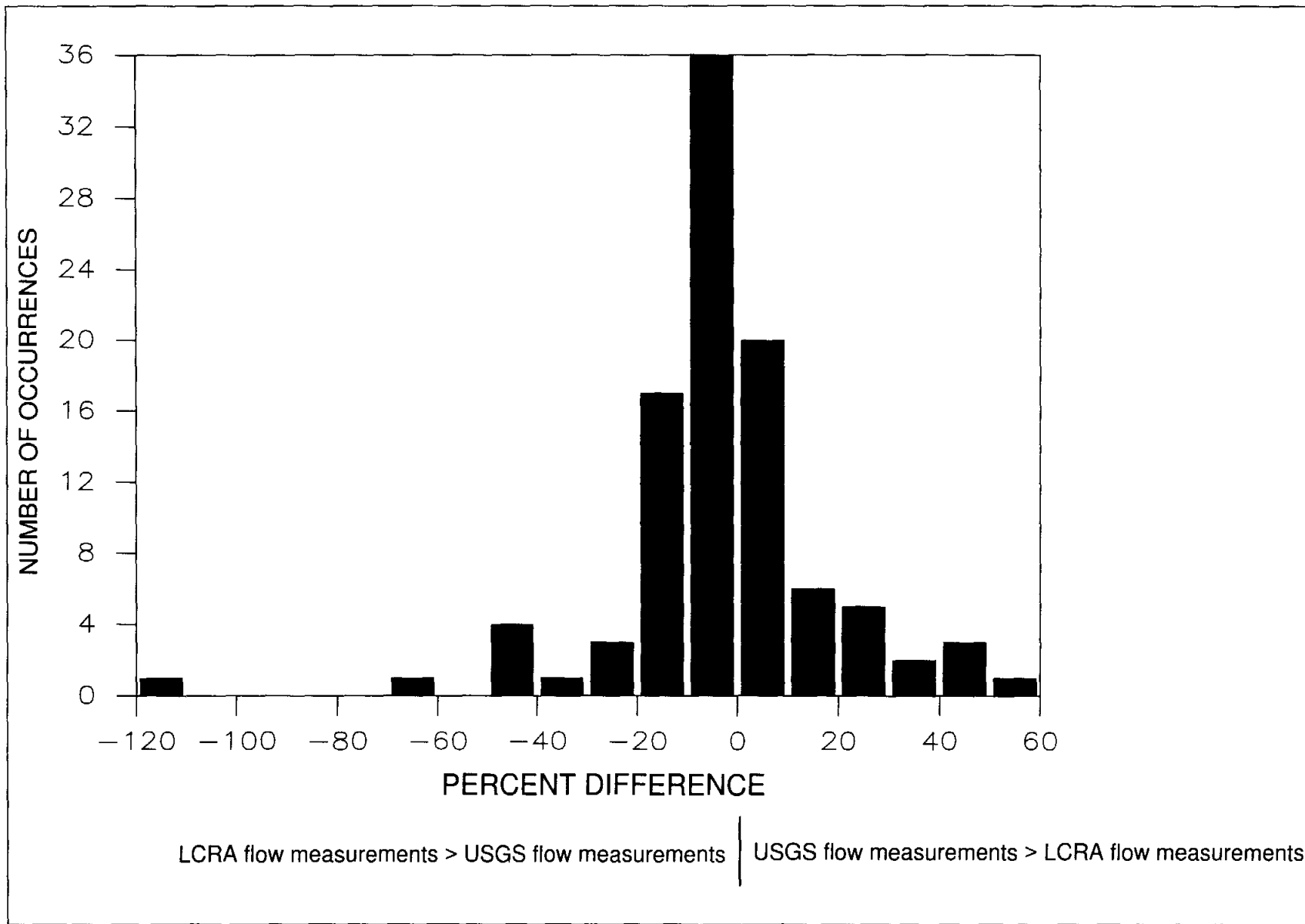
Figure 10. Histogram of percent differences between all Lower Colorado River Authority and U.S. Geological Survey flow measurements, Lakeside district.
