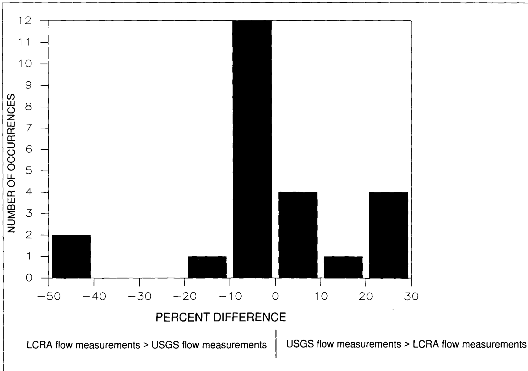
Figure 12. Histogram of percent differences between Lower Colorado River Authority and U.S. Geological Survey flow measurements made 1 hour or less apart, Lakeside district.
