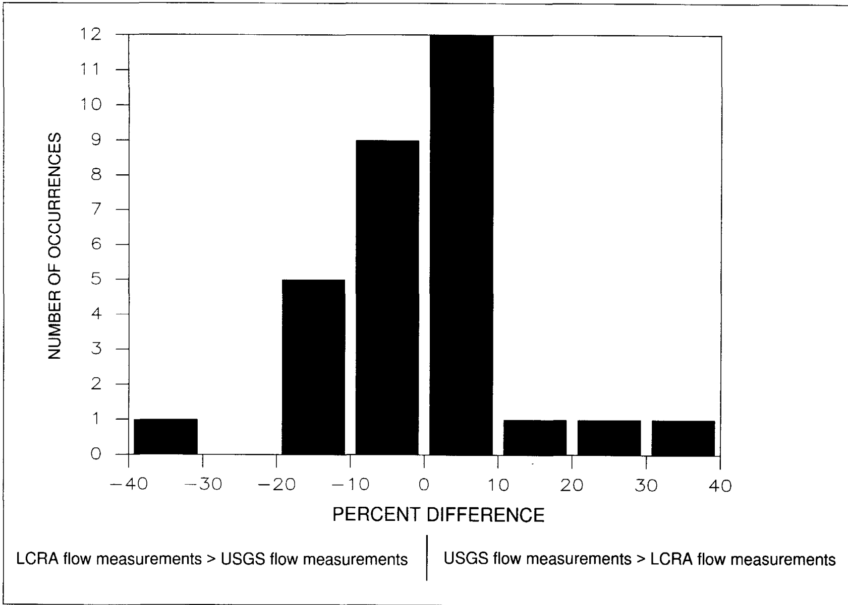
Figure 18. Histogram of percent differences between Lower Colorado River Authority and U.S. Geological Survey flow measurements made 1 hour or less apart, Gulf Coast district.
