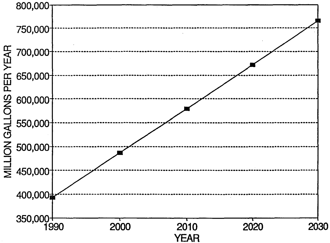
Figure IV-2 TOTAL WATER DEMAND PROJECTION FOR STUDY AREA
