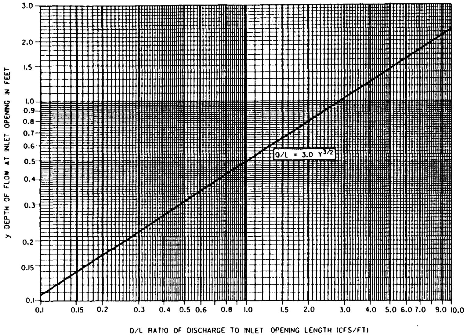
FIGURE 6-4 INLET CAPACITY
