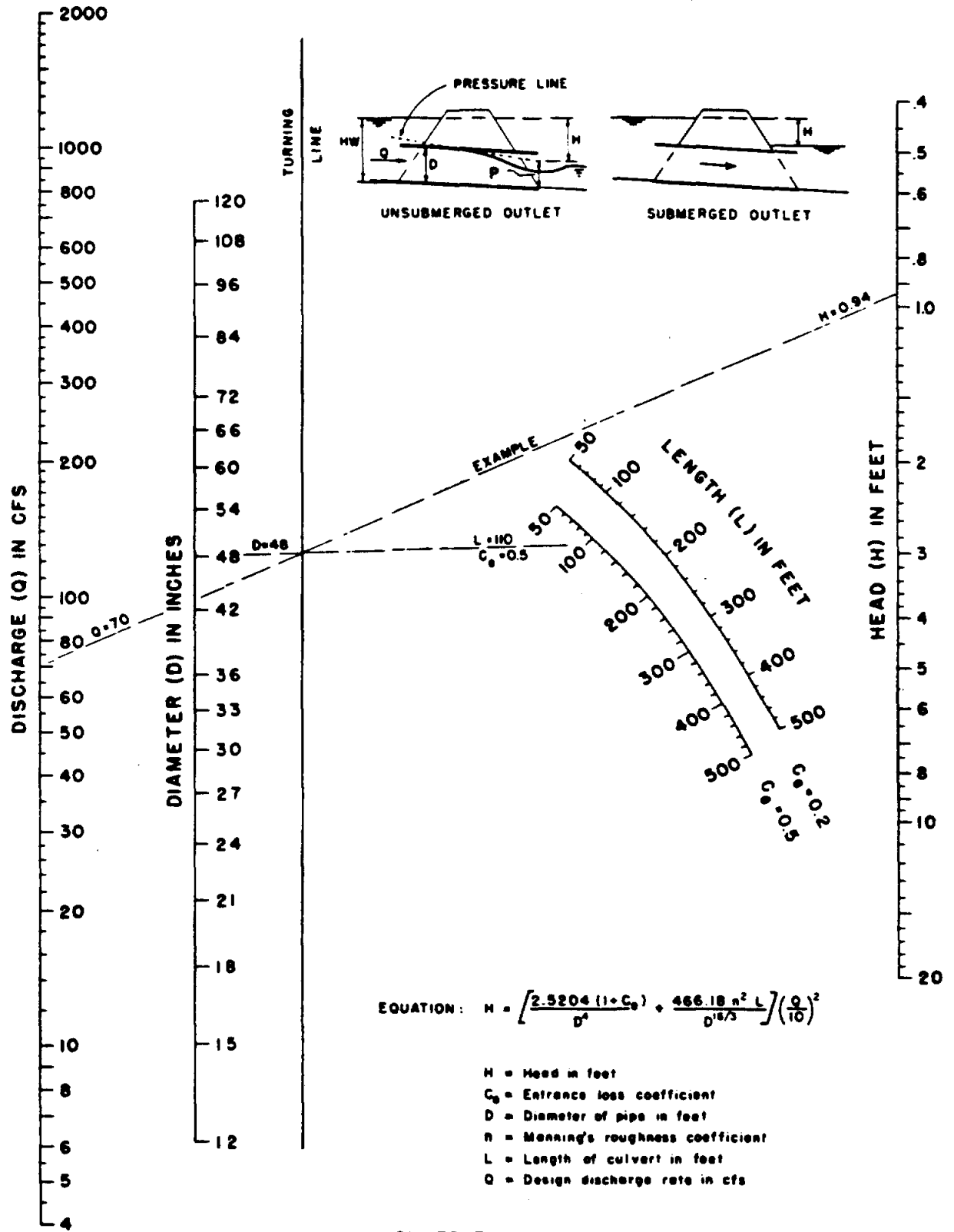
CHART 7-3 HEAD FOR CONCRETE PIPE CULVERTS FLOWING FULL
