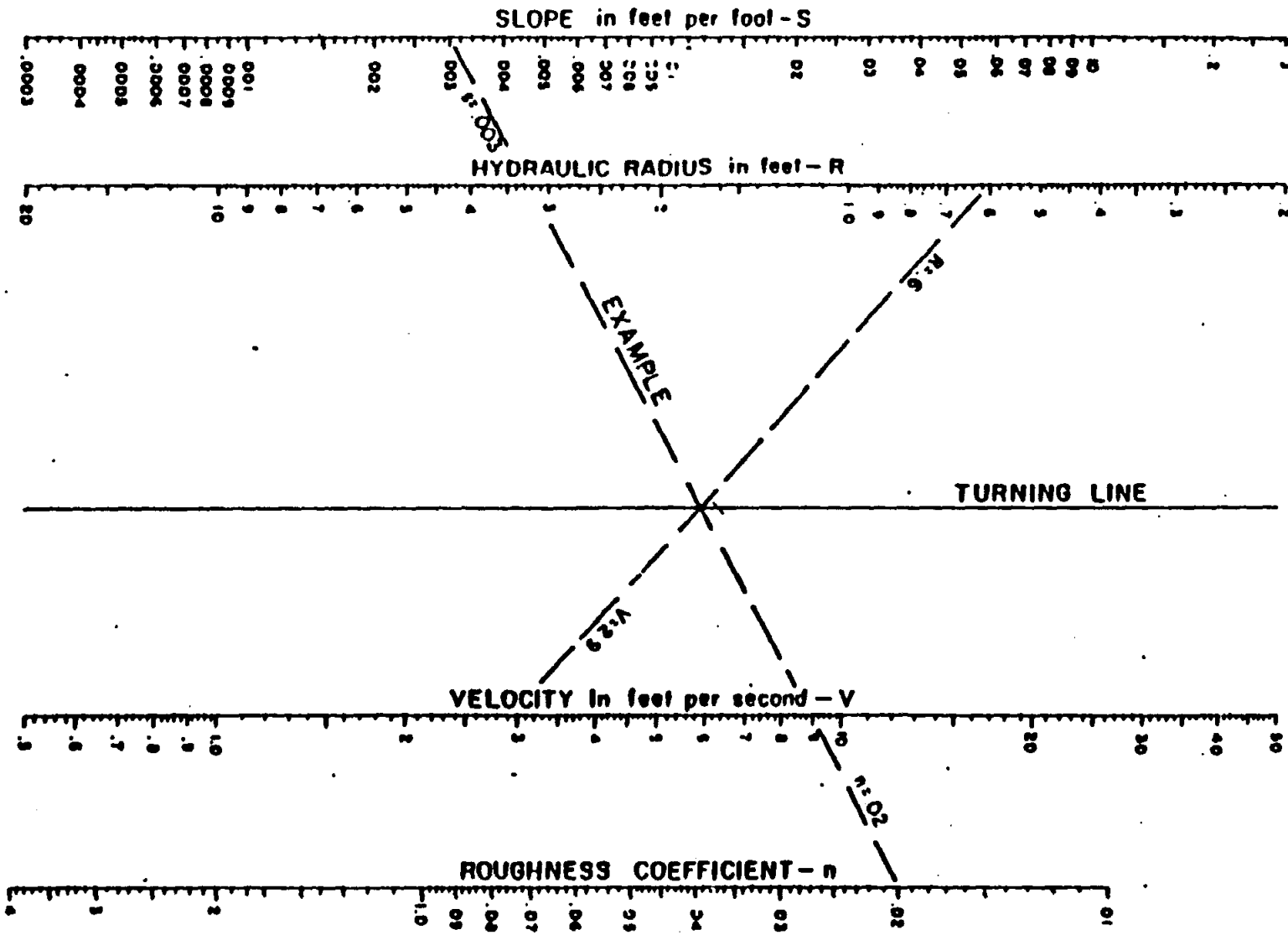
FIGURE 5-2 NOMOGRAPH FOR SOLUTION OF MANNING EQUATION
