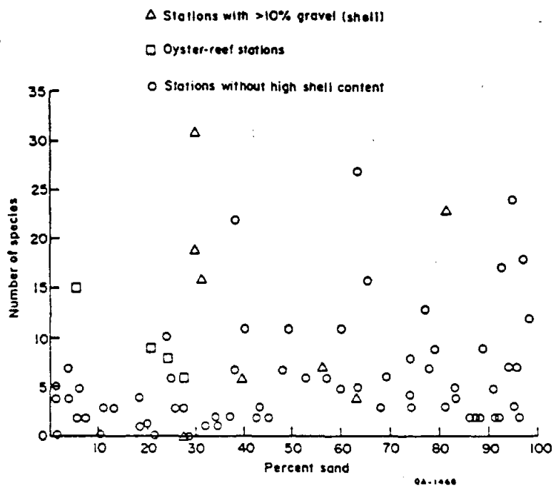
Figure 97. Scattergram of total species and percent sand in the bays of the Galveston–Houston area. (From White and others, 1985.)
