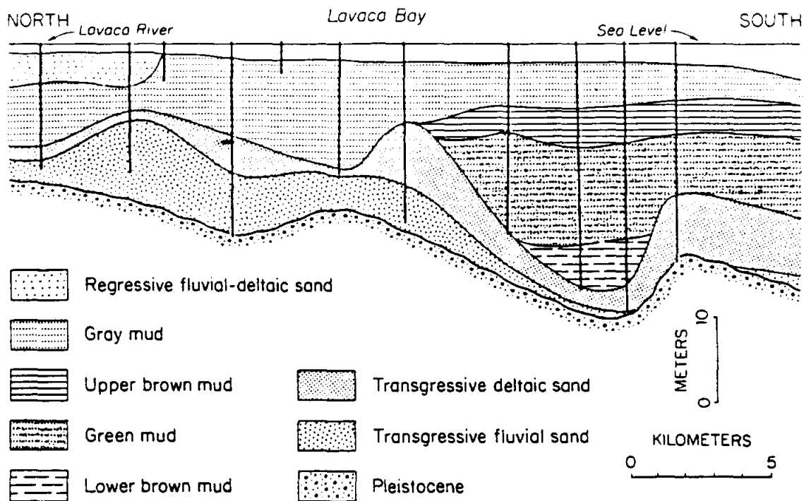
Figure 88. Cross section down Lavaca River valley showing sediments that have accumulated in Lavaca Bay above the Pleistocene surface. (From Wilkinson and Byrne, 1977; reprinted by permission.)
