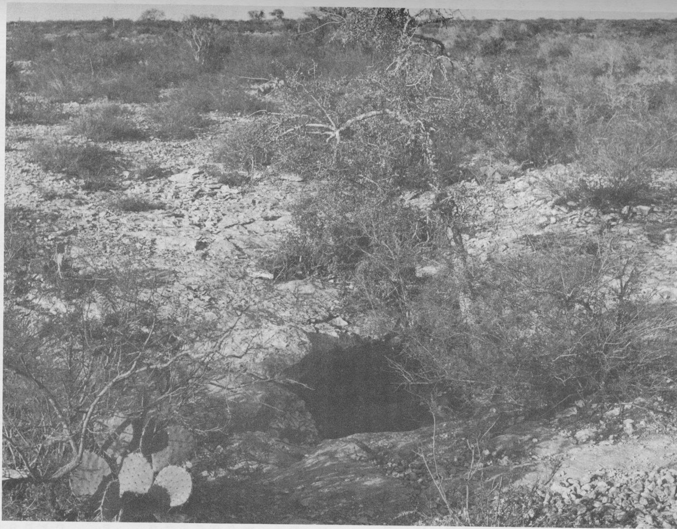
SOLUTIONAL OPENING IN THE AUSTIN CHALK, 4-1/2 MILES WEST OF BRACKETTVILLE AND ABOUT HALF A MILE SOUTH OF U.S. HIGHWAY 90
