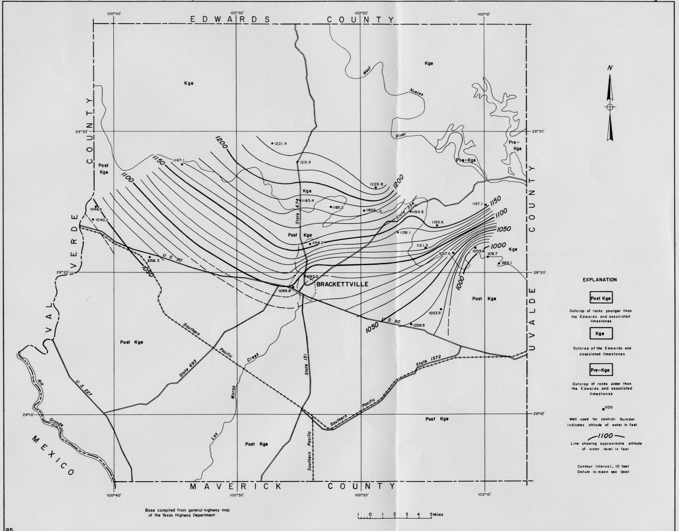
FIGURE 11.- Generalized geologic map of Kinney County, and configuration of the piezometric surface based on altitude of water levels in selected wells tapping the Edwards and associated limestones in August 1956
