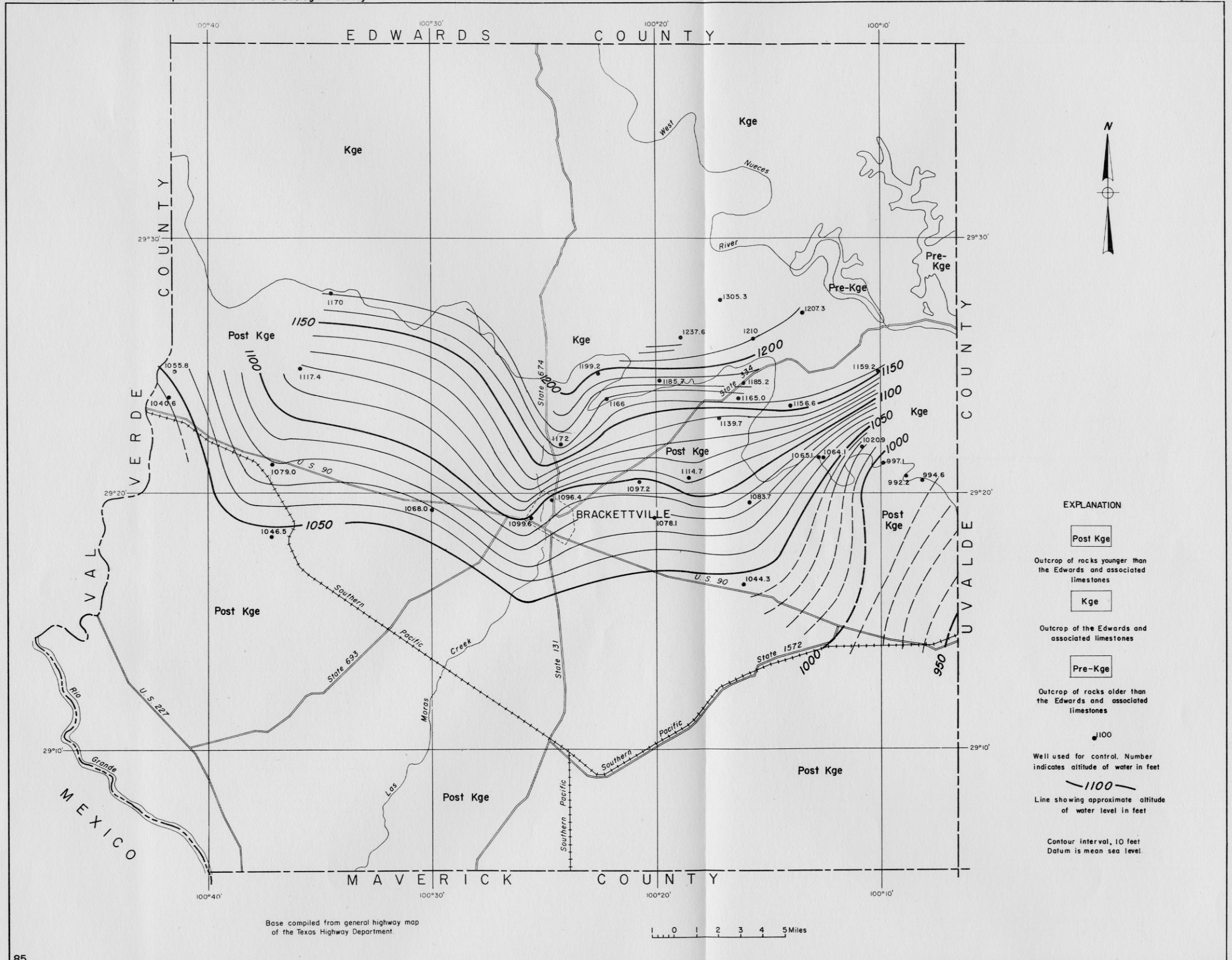
FIGURE 10.—Generalized geologic map of Kinney County, and configuration of the piezometric surface based on altitude of water levels in selected wells tapping the Edwards and associated limestones in January 1952
