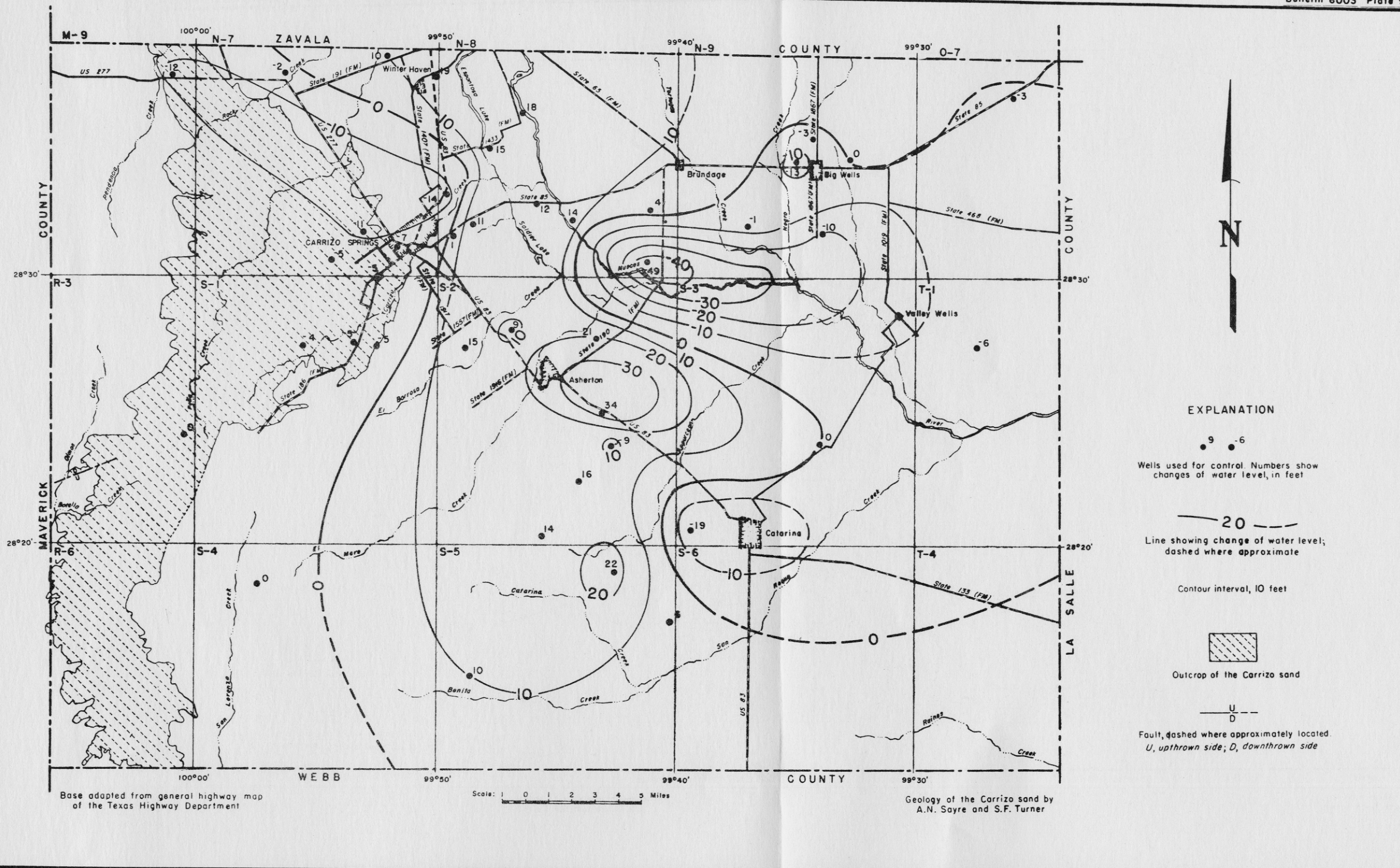
CHANGE IN WATER LEVELS IN WELLS IN THE CARRIZO SAND, DIMMIT COUNTY, TEXAS, 1929-38.
