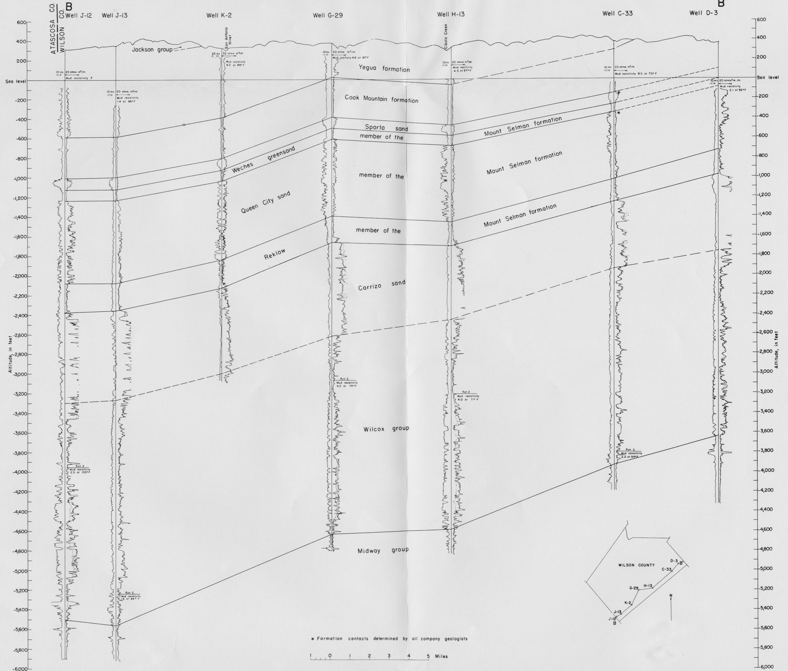
GEOLOGIC CROSS SECTION B-B', WILSON COUNTY, TEXAS.
