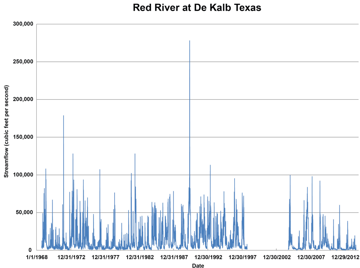
FIGURE 41. RED RIVER STREAMFLOW NEAR DE KALB TEXAS (SITE 07336820; U.S. GEOLOGICAL SURVEY, 2014C). 7
