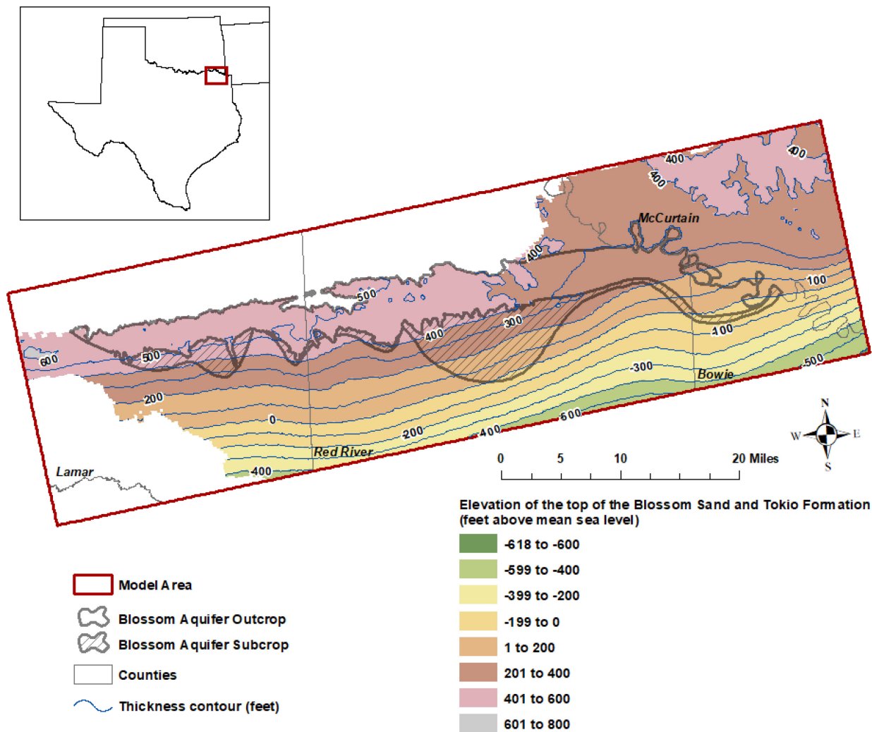
FIGURE 28. ELEVATION OF THE TOP OF LAYER THREE (THE BLOSSOM SAND).
