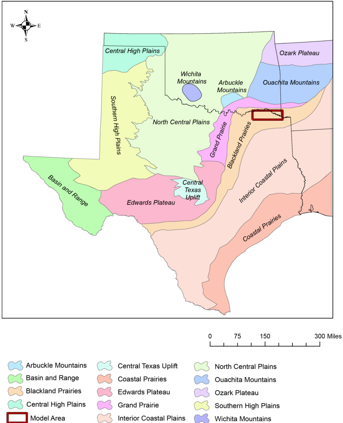
FIGURE 5. PHYSIOGRAPHIC PROVINCES IN TEXAS AND NEIGHBORING STATES (U.S. GEOLOGICAL SURVEY, 2014; FENNEMAN AND JOHNSON, 1946).
