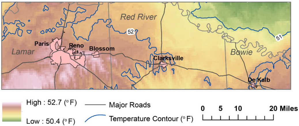
(c) Normal Daily Minimum Temperature
