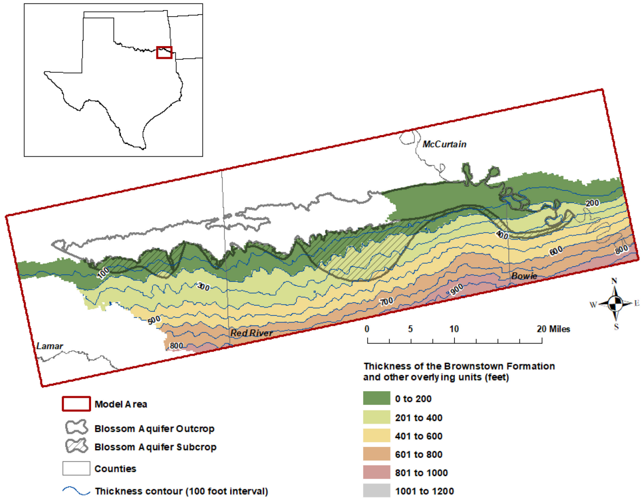
FIGURE 25. THICKNESS OF LAYER 2, THE BROWNSTOWN FORMATION AND OTHER OVERLYING UNITS 6 .
