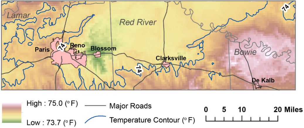
(b) Normal Daily Average Temperature
